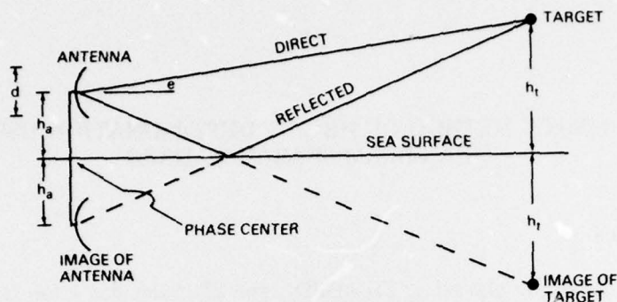
Fig. 1 — Multipath geometry
