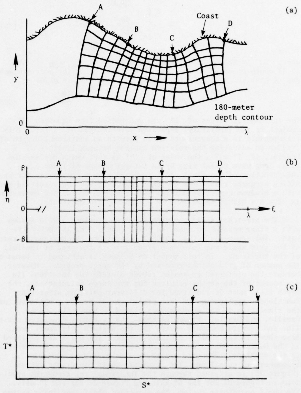
Figure 23. Orthogonal curvilinear grid system in the Z -plane (a), in the \zeta -plane (b), and in the computing grid (c).
