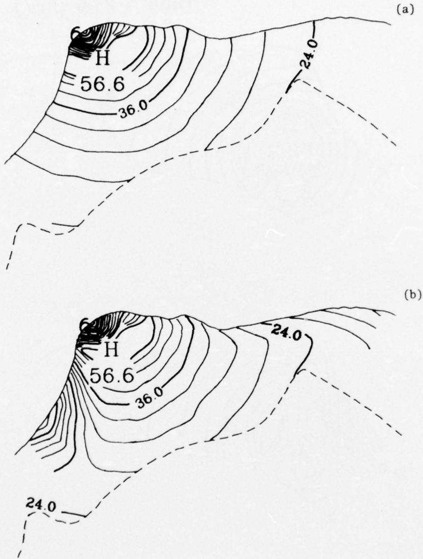
Figure 44. Hurricane Camille symmetric (a) and deformed (b) wind fields at 0400 G.m.t., 18 August 1969; isovels in meters per second.
