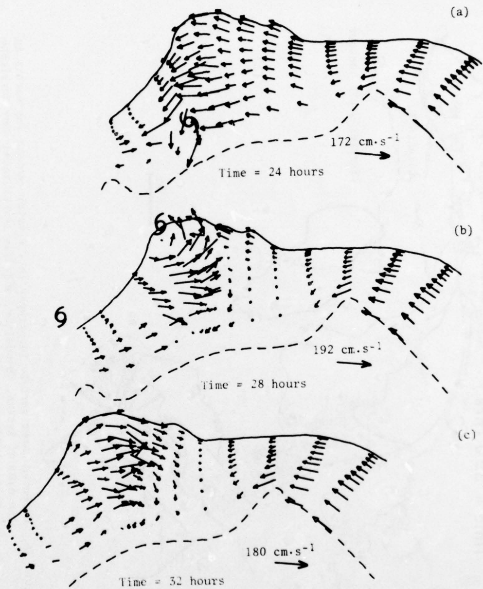
Figure 74. Computed water velocity in centimeters per second at selected grid points for Hurricane Camille at 24 (a), 28 (b), and 32 hours (c).
