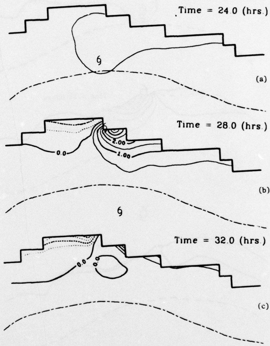
Figure 79. Computed water surface topography in 0.5-meter contour increments for Hurricane Gracie at 24 (a), 28 (b), and 32 hours (c), in the rectilinear grid.
