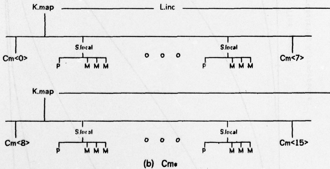
FIGURE 2.1 General structures of the two multiprocessor systems, C.mmp and Cm*
