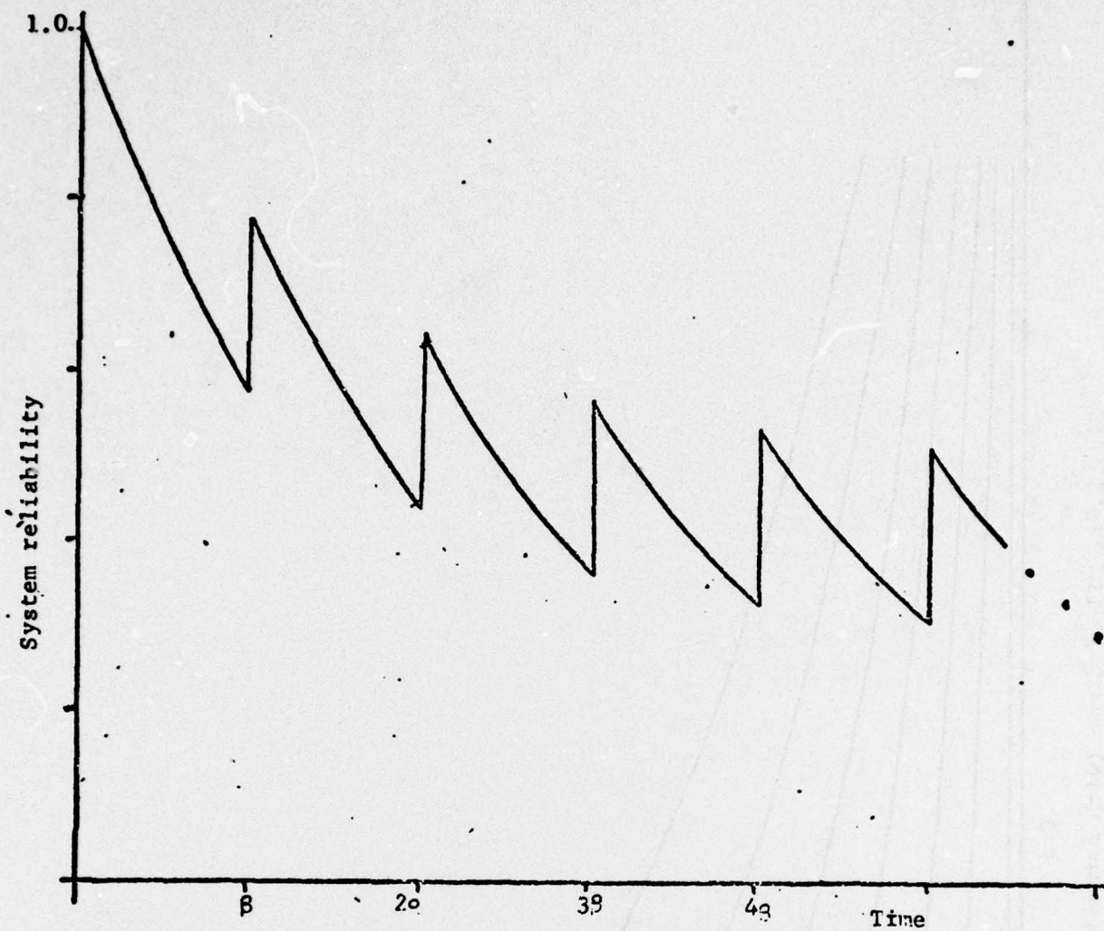
Figure 3.1: Effect of periodic maintenance on system reliability.
