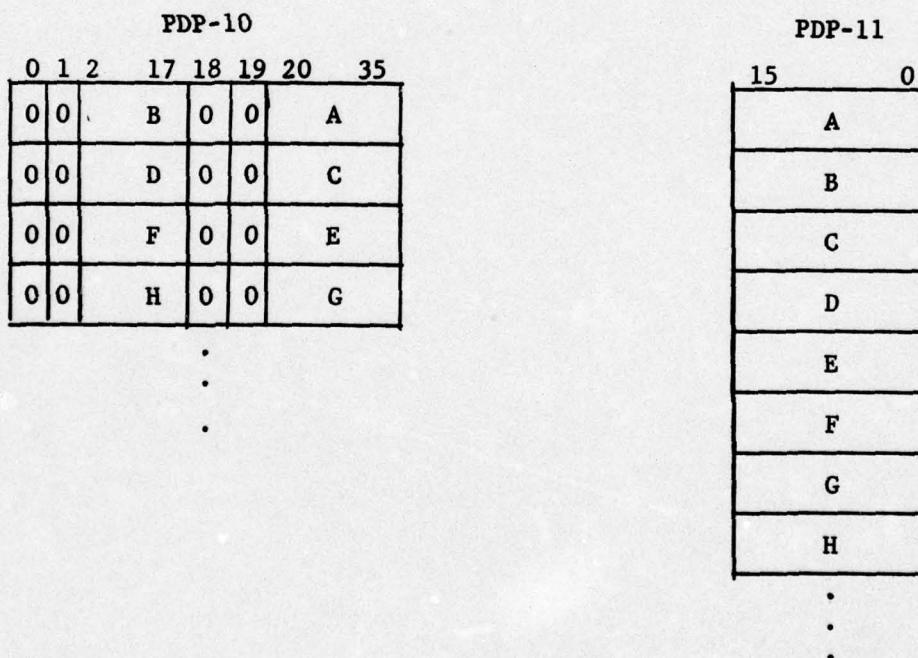
Figure 4-2. Data Packing Between the PDP-10 and PDP-11
