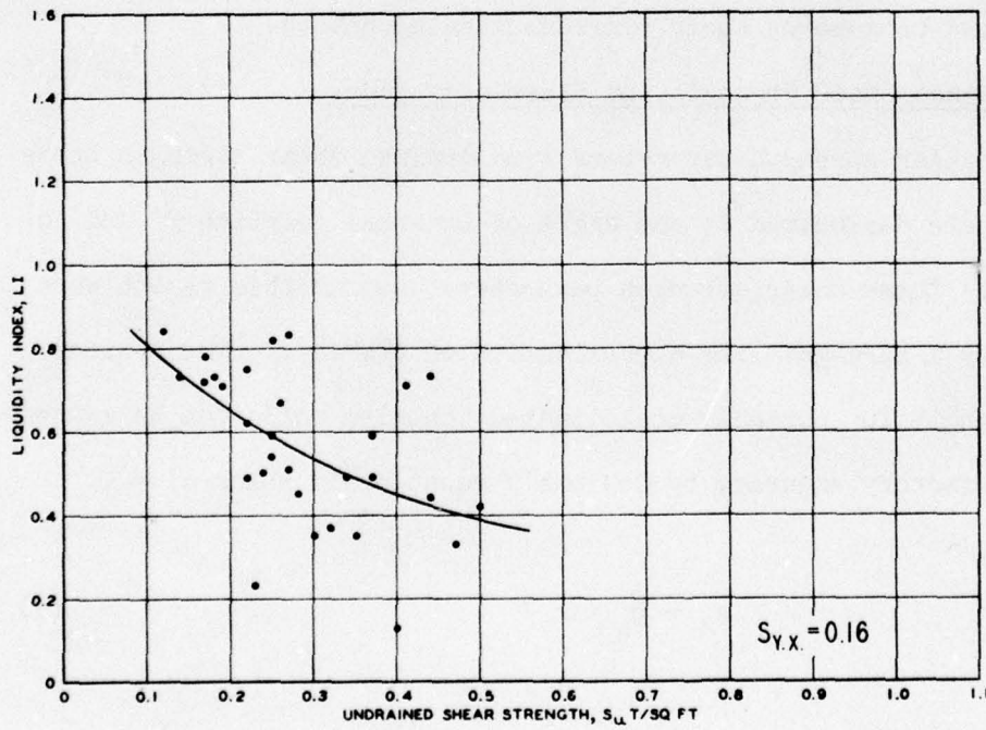
b. Intertributary
