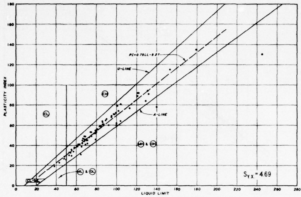
a. Interdistributary
