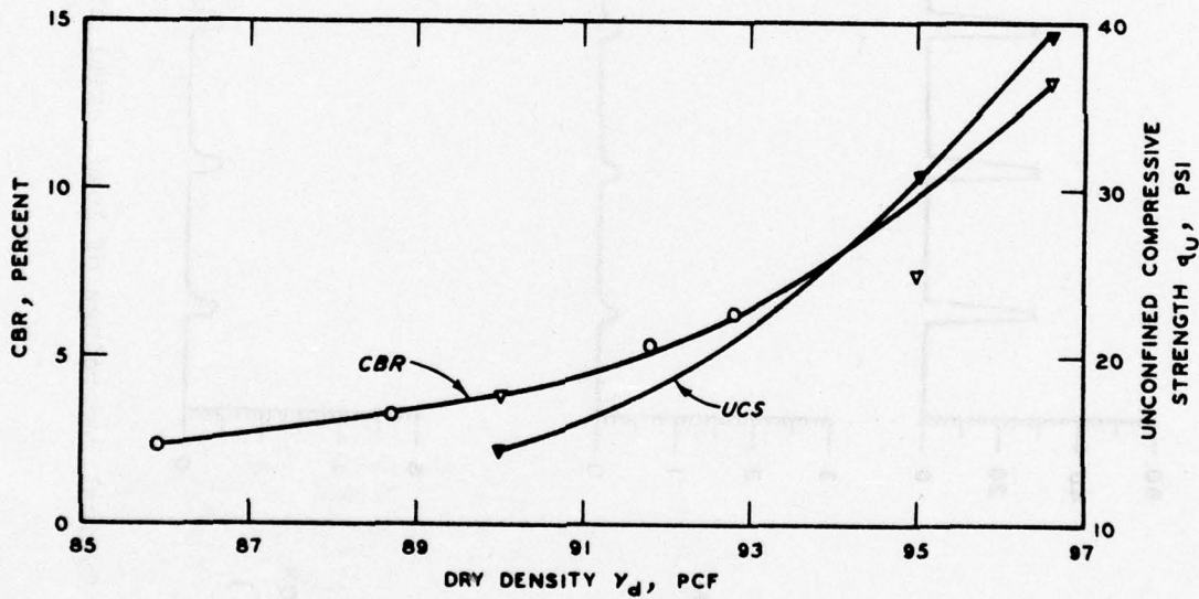
Figure 4. Effects of moisture content and density on CBR and UCS
