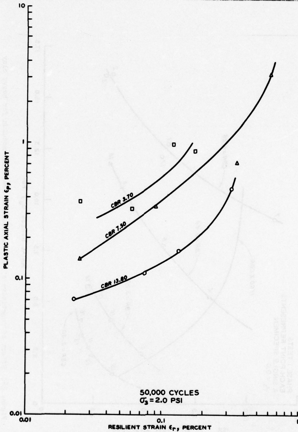
Figure 25. Relationship between plastic strain and resilient strain for heavy clay at 50,000 repetitions
