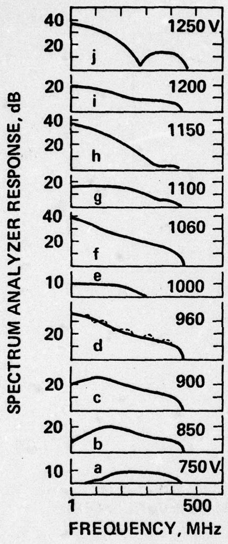
SPECTRAL OUTPUT FOR VARIOUS STARK BIASES
