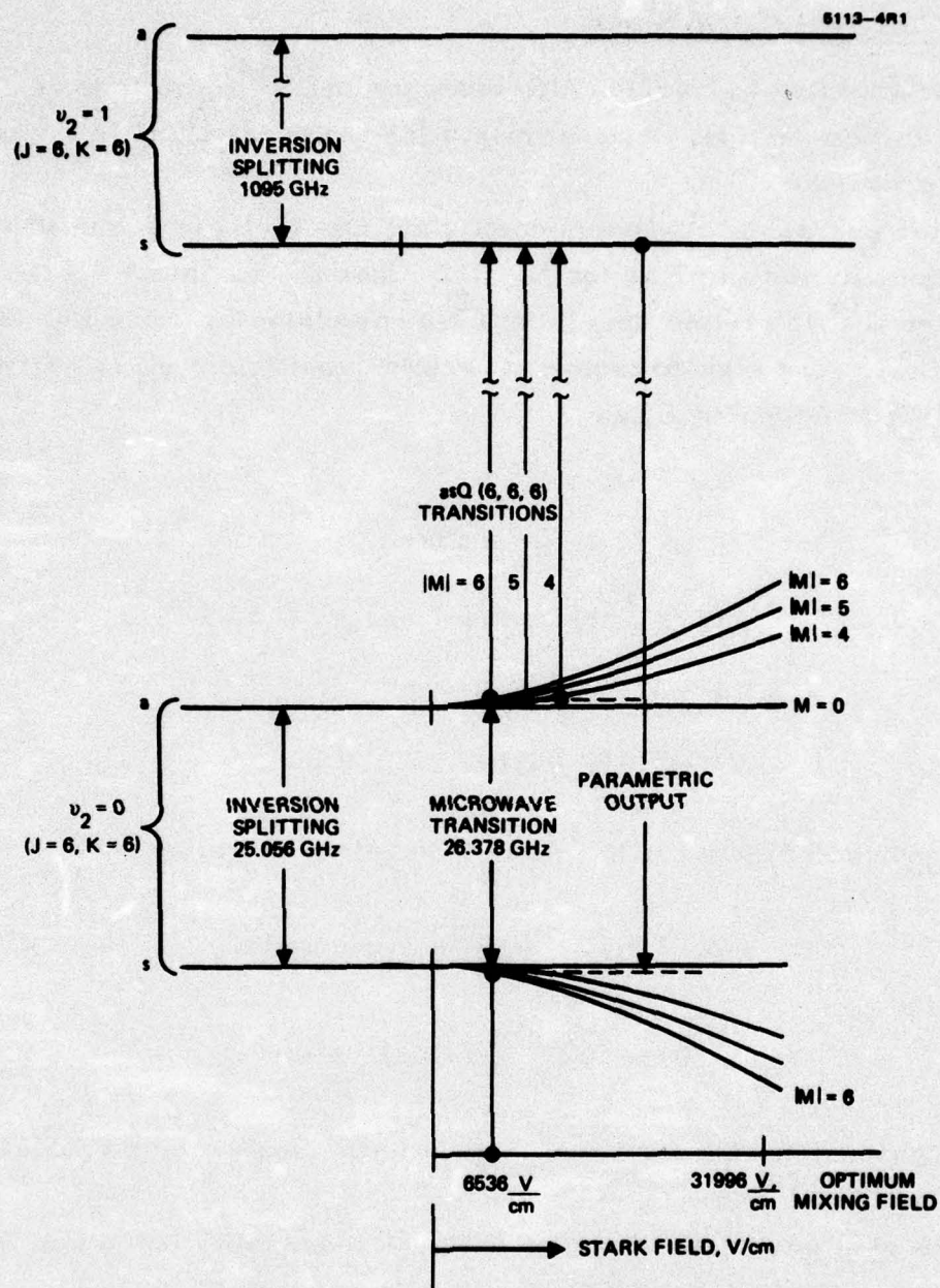
Figure 3. Energy levels of N^{14}H_3 involved in the resonant parametric interaction. The C^{13}O_2^{16}R(18) laser line is resonant with the asQ(6,6,6) transition. The parametric output is up-converted. The s \rightarrow s transition is forbidden in this symmetric top with zero Stark field. The |M| = 6, 5, 4, \Delta M = 0 transitions are indicated, corresponding to the absorption lines of Figure 1.
