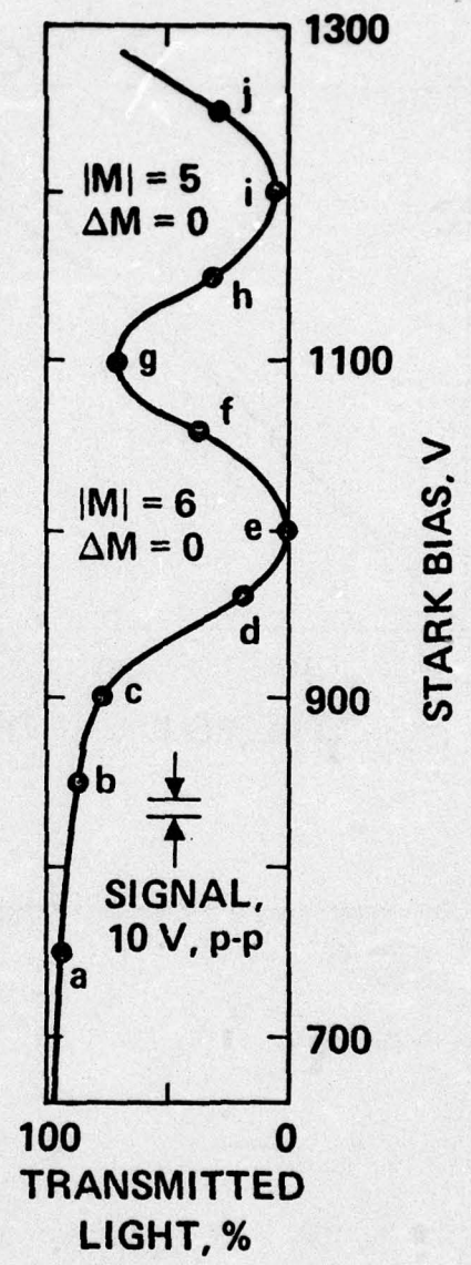
ABSORPTION SPECTRUM vs STARK BIAS
