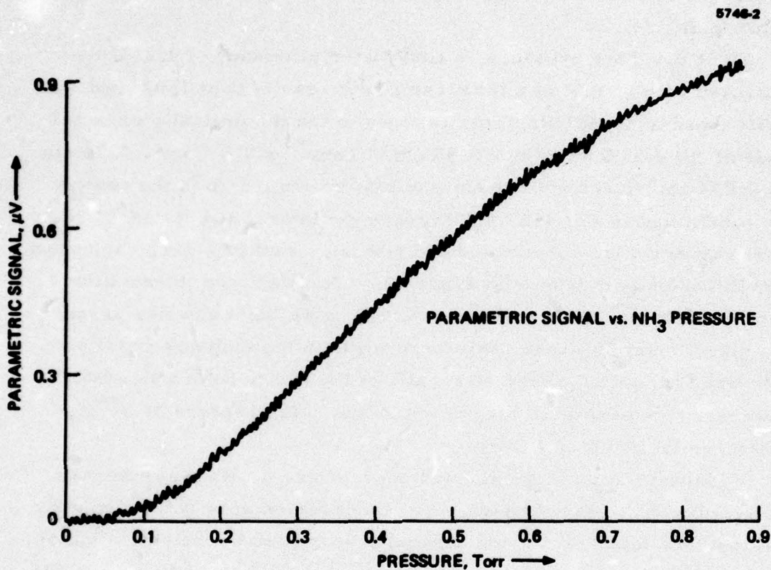
Figure 6. Parametric signal (detector output) versus N 14 H 3 pressure for the single pass microwave cavity. Electrical breakdown occurred intermittently between 0.7 and 0.9 Torr. The curve indicates saturation at higher pressures due to pressure broadening; the curve is also dependent upon the absorption of the optical waves.
