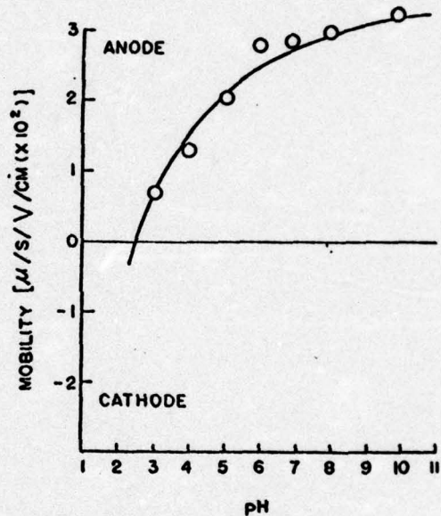
FIG. 2. Relationship between pH and mobility of glutaraldehyde-fixed, sonically freed P. berghei . Glutaraldehyde fixation did not much affect the charge characteristics of the parasites, which indicates that amino and guanidinium groups do not contribute significantly to the charge characteristics of the parasites.
