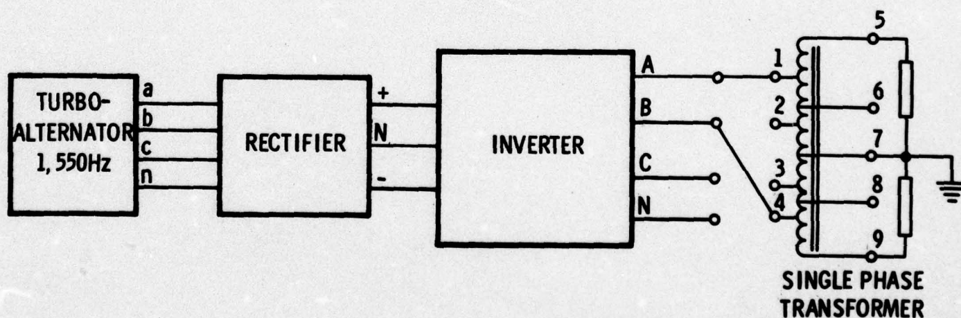
Figure 2-43. Connections for 60 Hz, Single-Phase, Three-Wire Power
