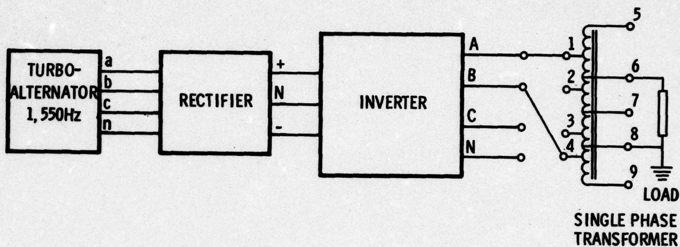
Figure 2-42. Connections for 60 Hz, Single-Phase, Two-Wire Power
