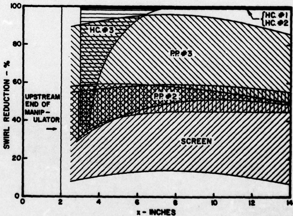
Figure 7. Swirl Reduction in Different Test Flow Conditions for One Flow Manipulator and Composite of Reduction Range for Several Manipulators.
