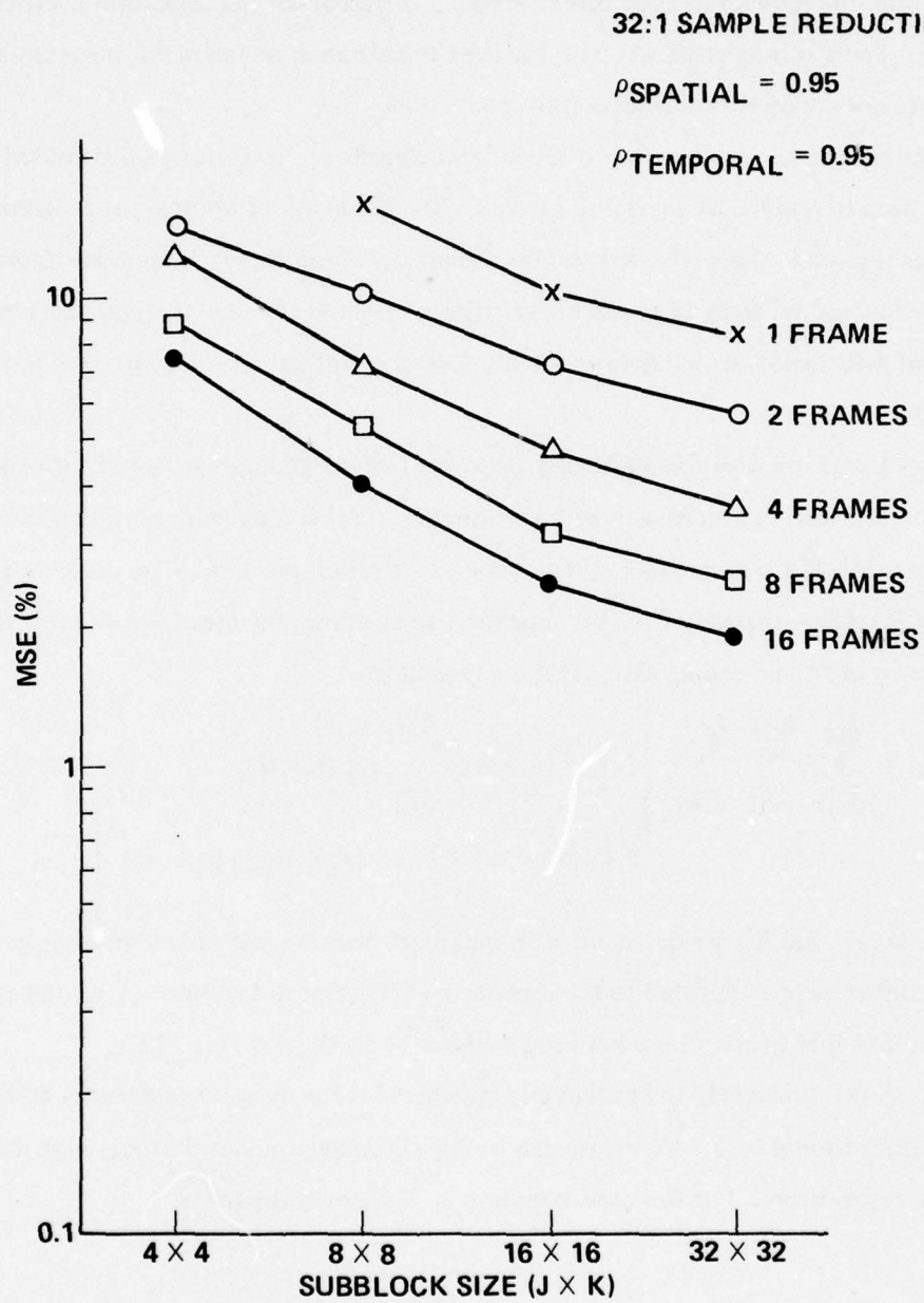
Figure 3-6. Theoretical Performance Evaluation for Three-Dimensional Cosine Transform Coder with Zonal Sampling
