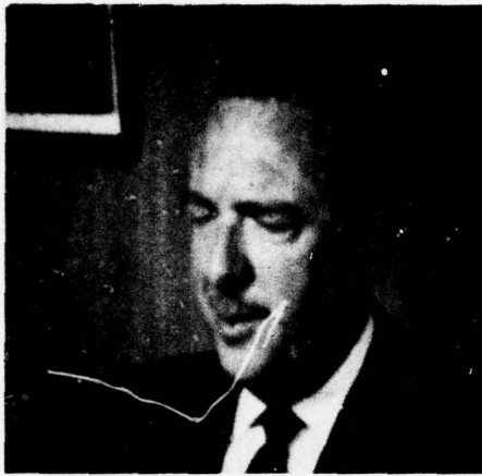
(a) 1.0 bits/pixel/frame
