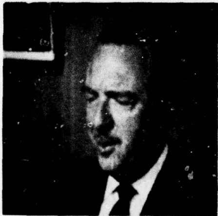
(c) 0.25 bits/pixel/frame
