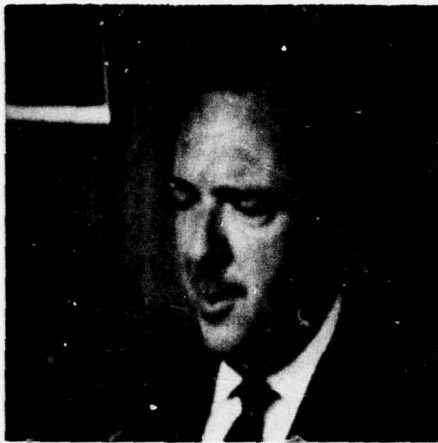
(a) 1.0-bits/pixel/frame
