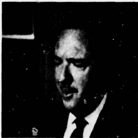
(a) 2.0 bits/pixel
