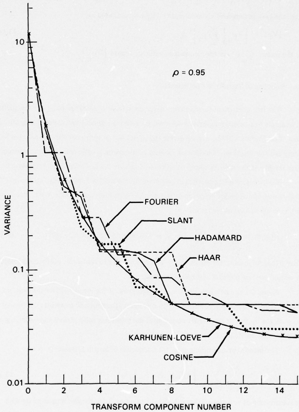
Figure 3-4. Comparison of Transform Domain Variance Functions
