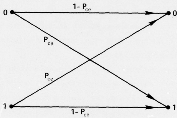
Figure 5-1. Binary Symmetric Channel Model
