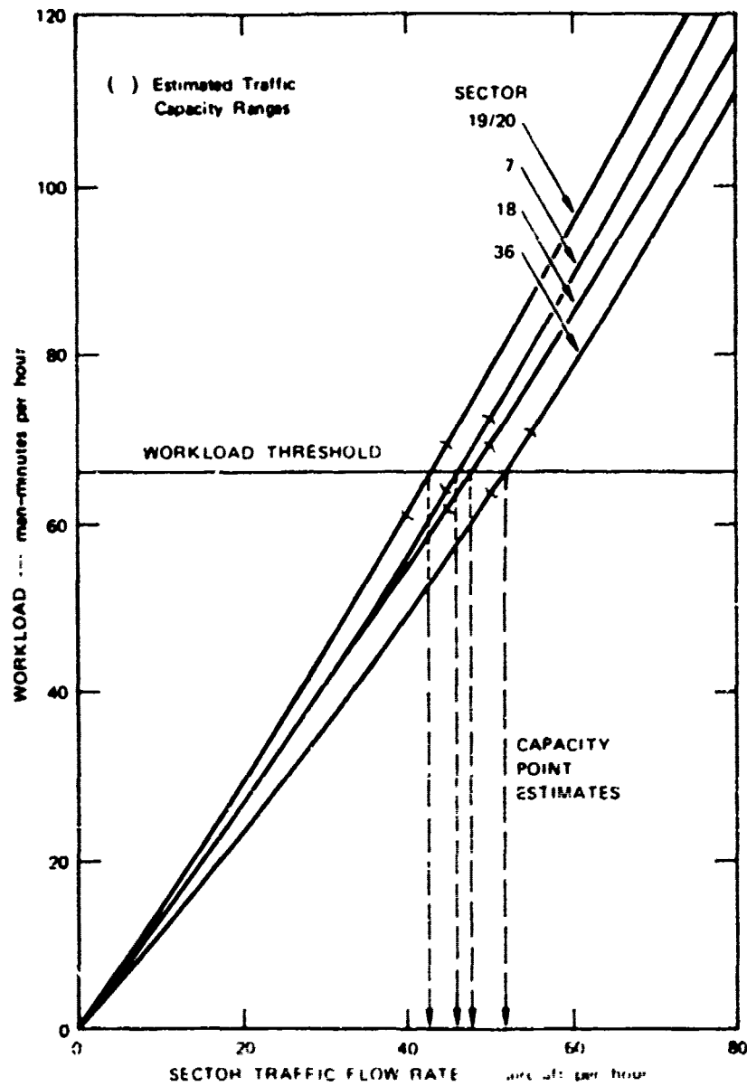
FIGURE 2 SECTOR TEAM WORKLOAD CALIBRATION
