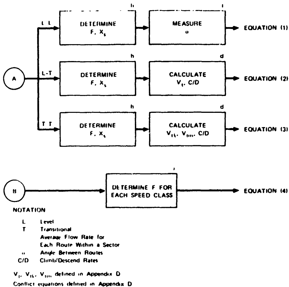
FIGURE 8 RECEP DATA COLLECTION AND REDUCTION ON POTENTIAL CONFLICT EVENTS MAJOR STEPS (Concluded)
