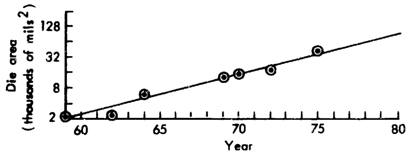
Fig. B.2--Increase in die area for most complex integrated devices commercially available
