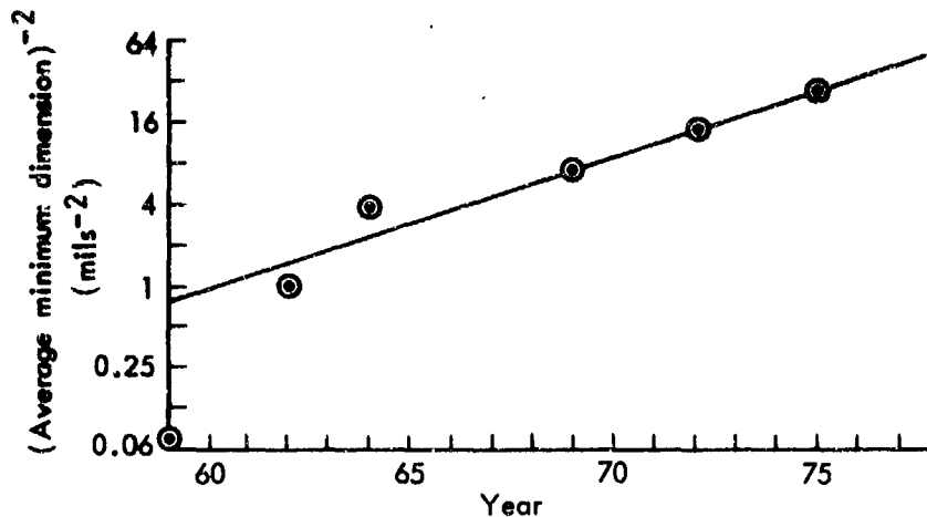
Fig. B.3--Device density contribution from the decrease in line widths and spacings
