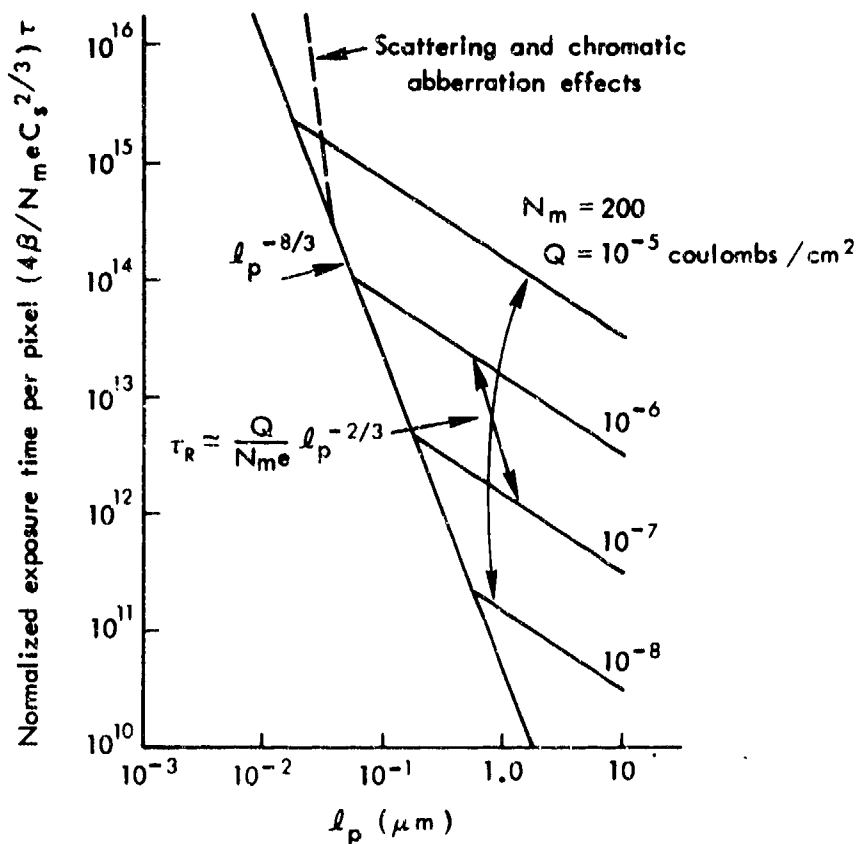
Fig. 2--Normalized exposure time/pixel vs pixel dimension
