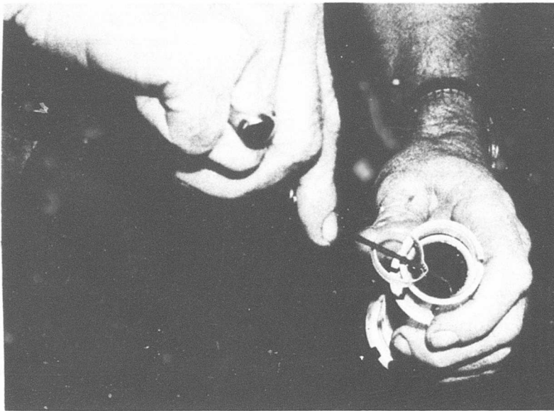
Figure 29. Use of pick to remove hydraulic actuator O-ring seals.
