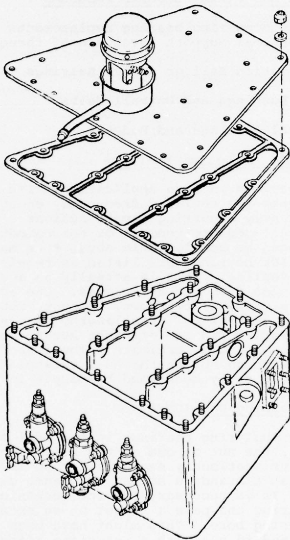
Figure 35. Reservoir cover attachment studs, CH-47 combining transmission.
