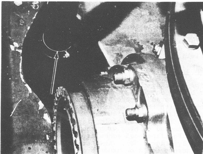
Figure 57. "Bottomed-out" boot clamp, UH-1 hydraulic actuator.
