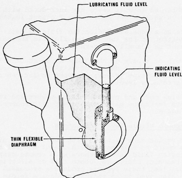
Figure 54. Sight gauge with segregated indicating fluid.
