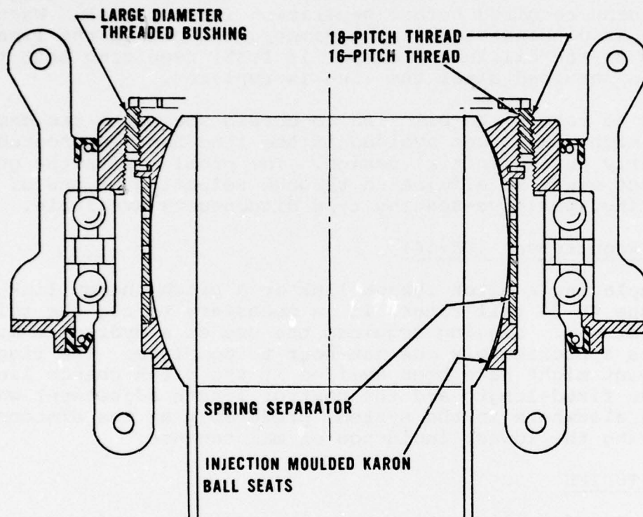
Figure 42. Swashplate uniball with threaded seats.
