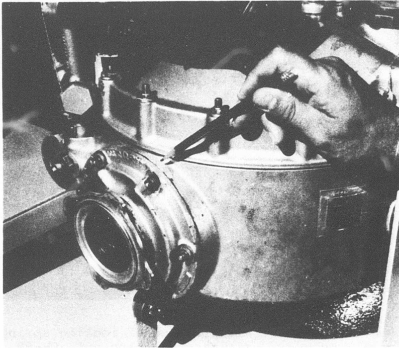
Figure 9. Location of laminated shims behind input bearing/seal housing, OH-58 transmission.
