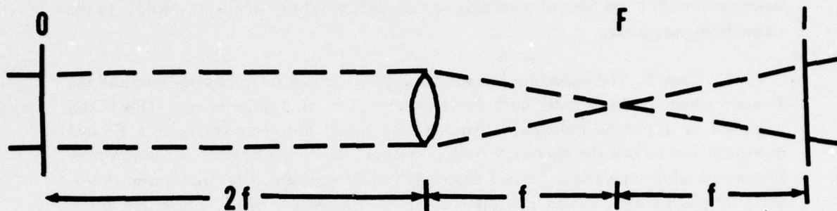
Figure 8. Imaging Geometry
