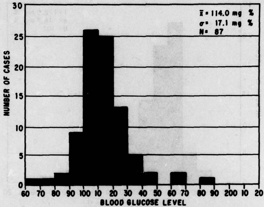
FIGURE 5 Distribution of blood glucose levels. Postflight values in those flying the second period only.
