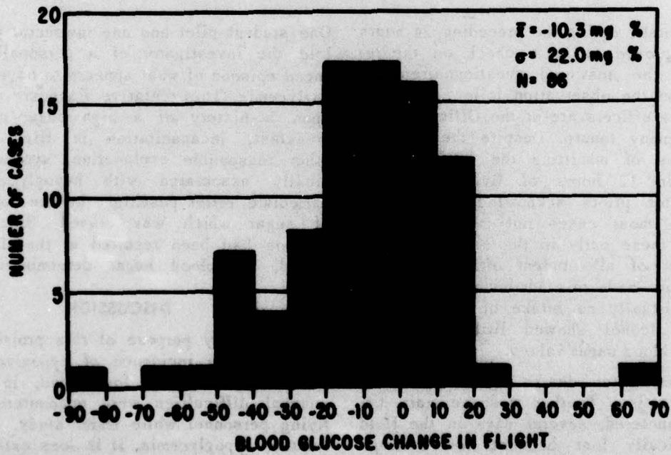
FIGURE 6 Distribution of in-flight changes in blood glucose levels. Changes in those flying the second period only.
