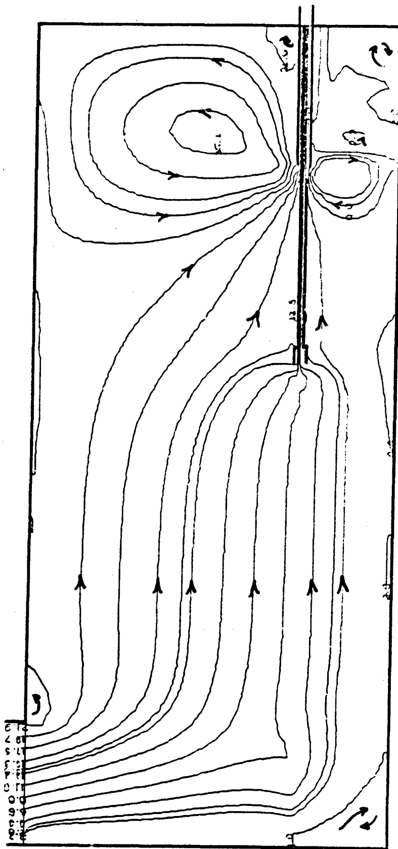
FIGURE 9. DISTRIBUTION OF STREAMLINES RUN G1: 100% RPM, AUGMENTATION RATIO = 1.0:1.
