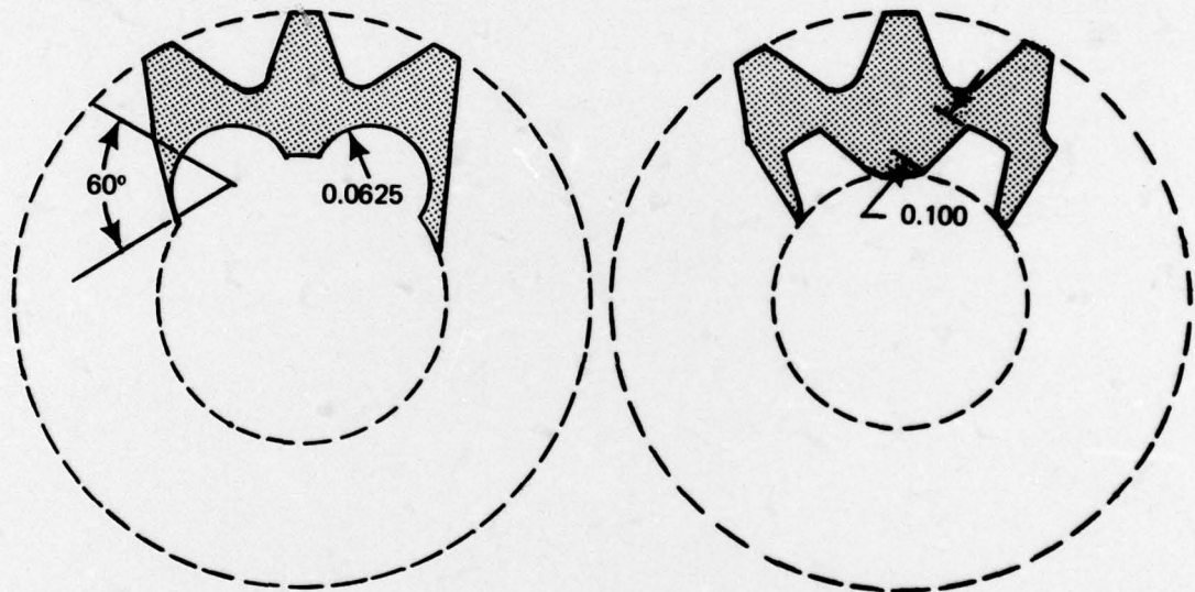
TOOTH ARC LENGTH = 0.065 (CIRCULAR TOOTH)
