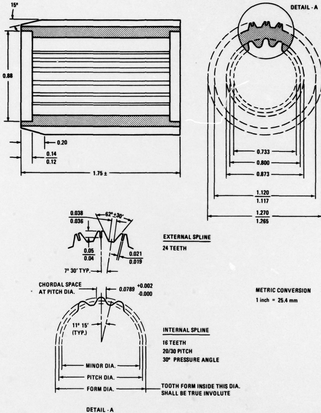
Figure 17 Proposed Polyimide Plastic Involute Spline Adapter
