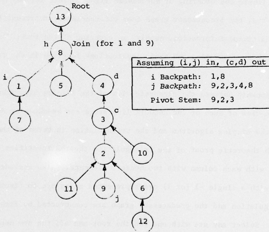
Figure 2. A Transshipment Basis (for Figure 1).
