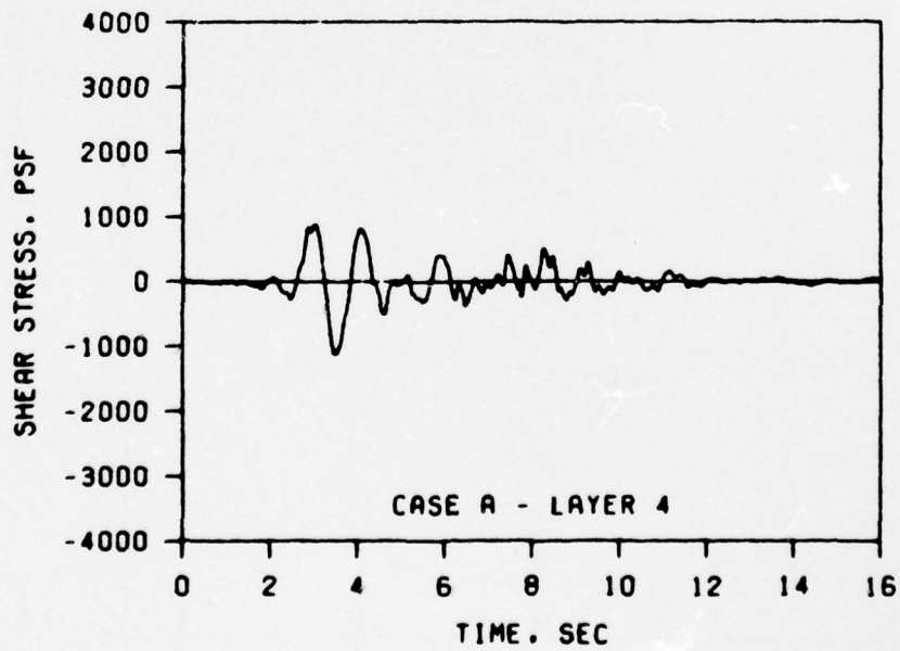
Figure 8. Shear stress-time histories for the tops of layers 2 and 4, Case A
