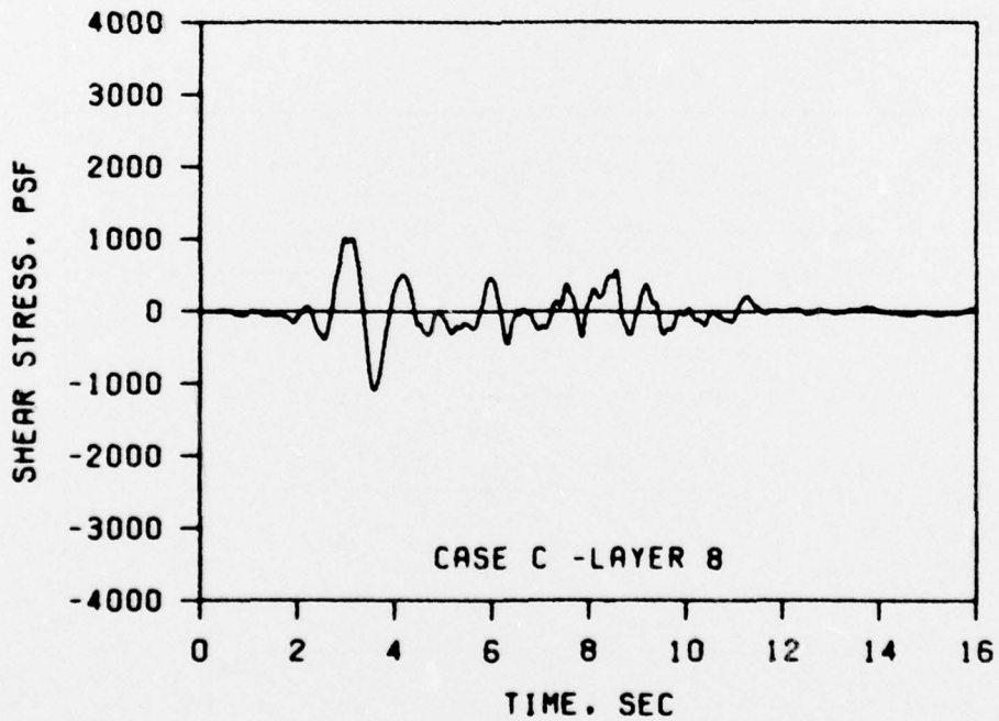
Figure 18. Shear stress-time histories for the tops of layers 6 and 8, Case C (Kentucky abutment)
