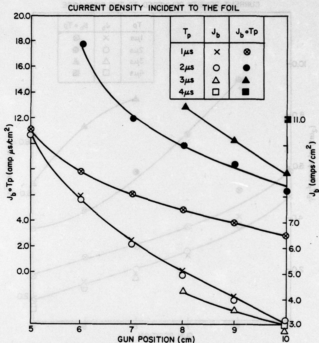
Fig. 3 — Plot of the current density J_b incident to the foil (25 \mu m titanium) for 1 \mu sec ( \times ) 2 \mu sec ( \circ ) 3 \mu sec ( \triangle ) and 4 \mu sec ( \square ) pulses at a gun voltage of 300 kV. Charge density ( J_b \cdot t ) is also plotted. Measurements were made with a current density button.
