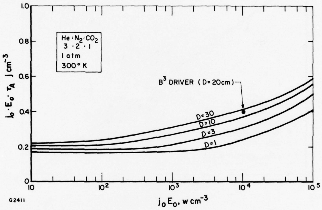
Fig. 15a Loading Energy at Streamer Transit in Discharge at 1 atm
