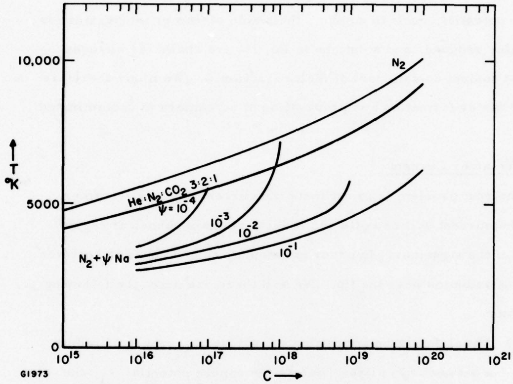
Fig. 7 Solution to Equation (5) for T as Function of C
