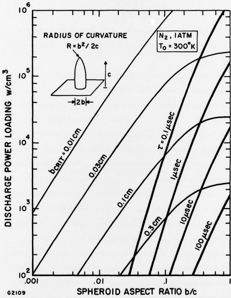
Fig. 16 Streamer Critical Radius and Latent Period for Spheroidal Protrusion
