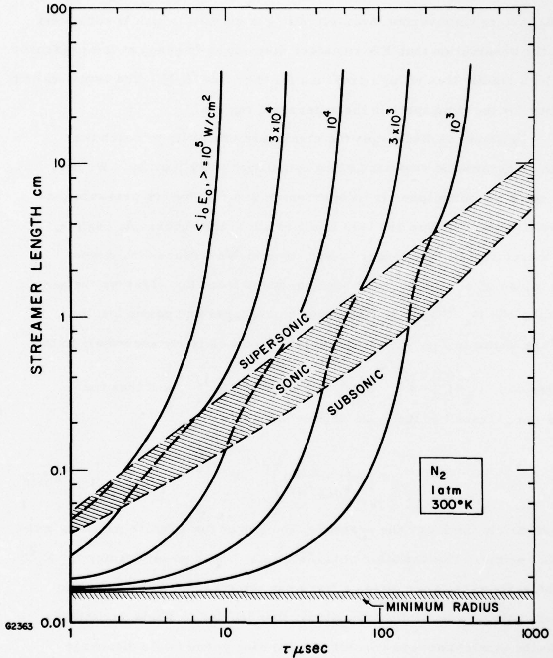
Fig. 9 Streamer Length vs Time
