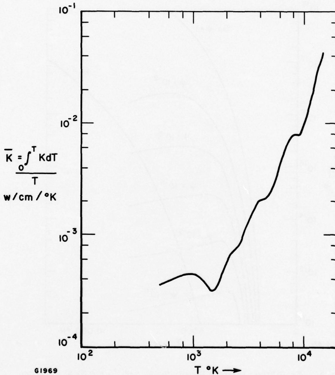
Fig. 6 Mean Thermal Conductivity for Air. This can be approximated as \bar{K} = 3.145 \times 10^{-10} T^{1.893} , T in °K for 1500 < T < 15,000 .
