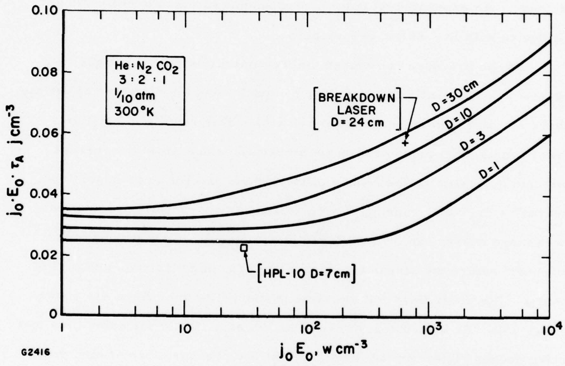
Fig. 15b Loading Energy at Streamer Transit in Discharge at 1/10 atm
