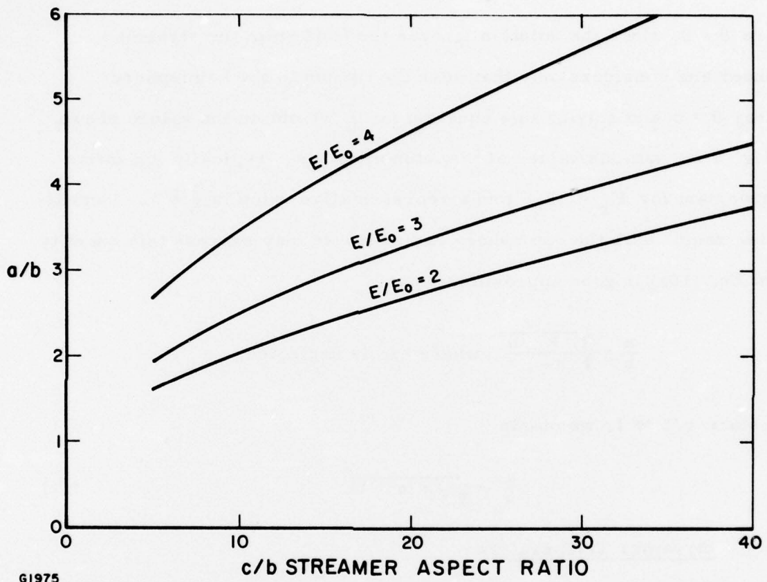
Fig. 8 Ratio of Cap Sphere to Cylinder Radius for Streamers, as Function of Aspect Ratio
