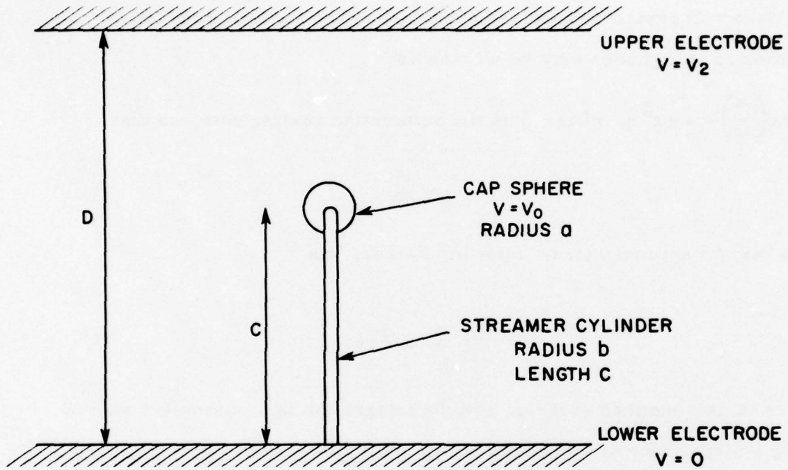
Fig. 4 Model for Streamer Propagation
