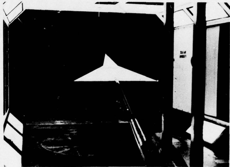
FIG. 3 SURFACE FLOW AR4-A1 WING
