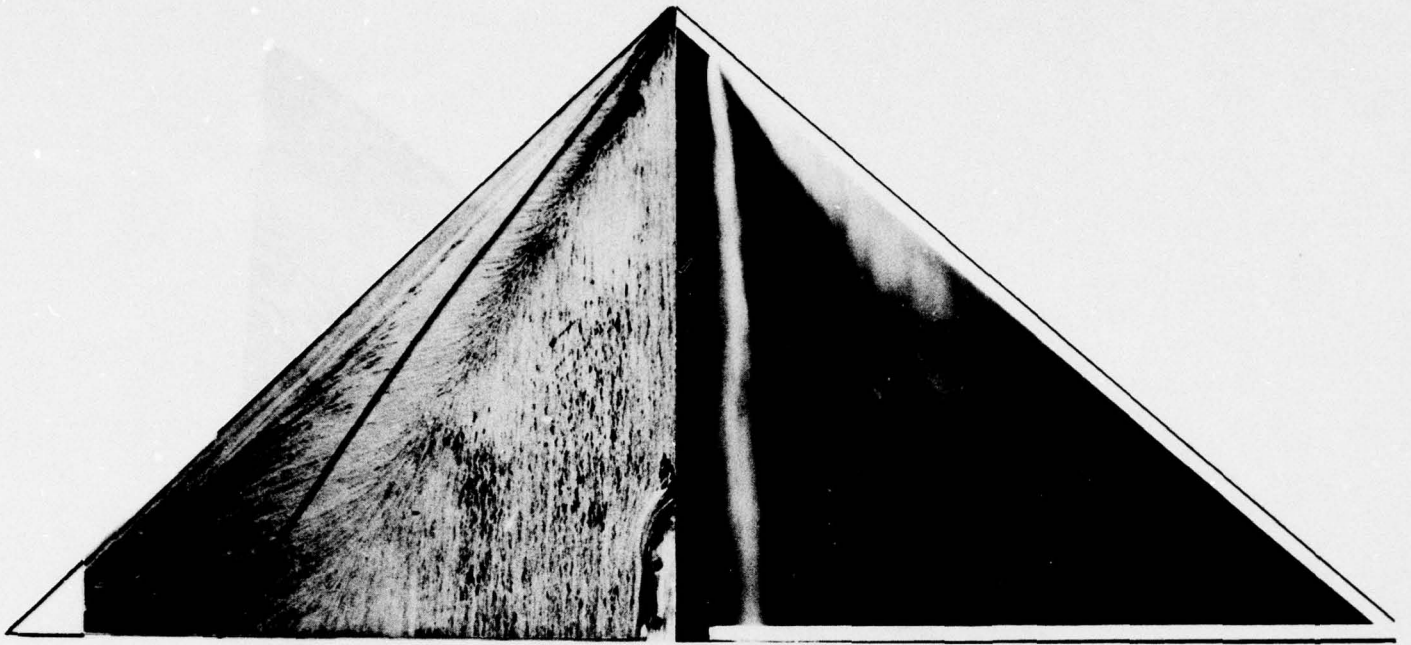
FIG. 11a SURFACE FLOW PATTERN AND VORTEX STRUCTURE OVER AR4 WING
