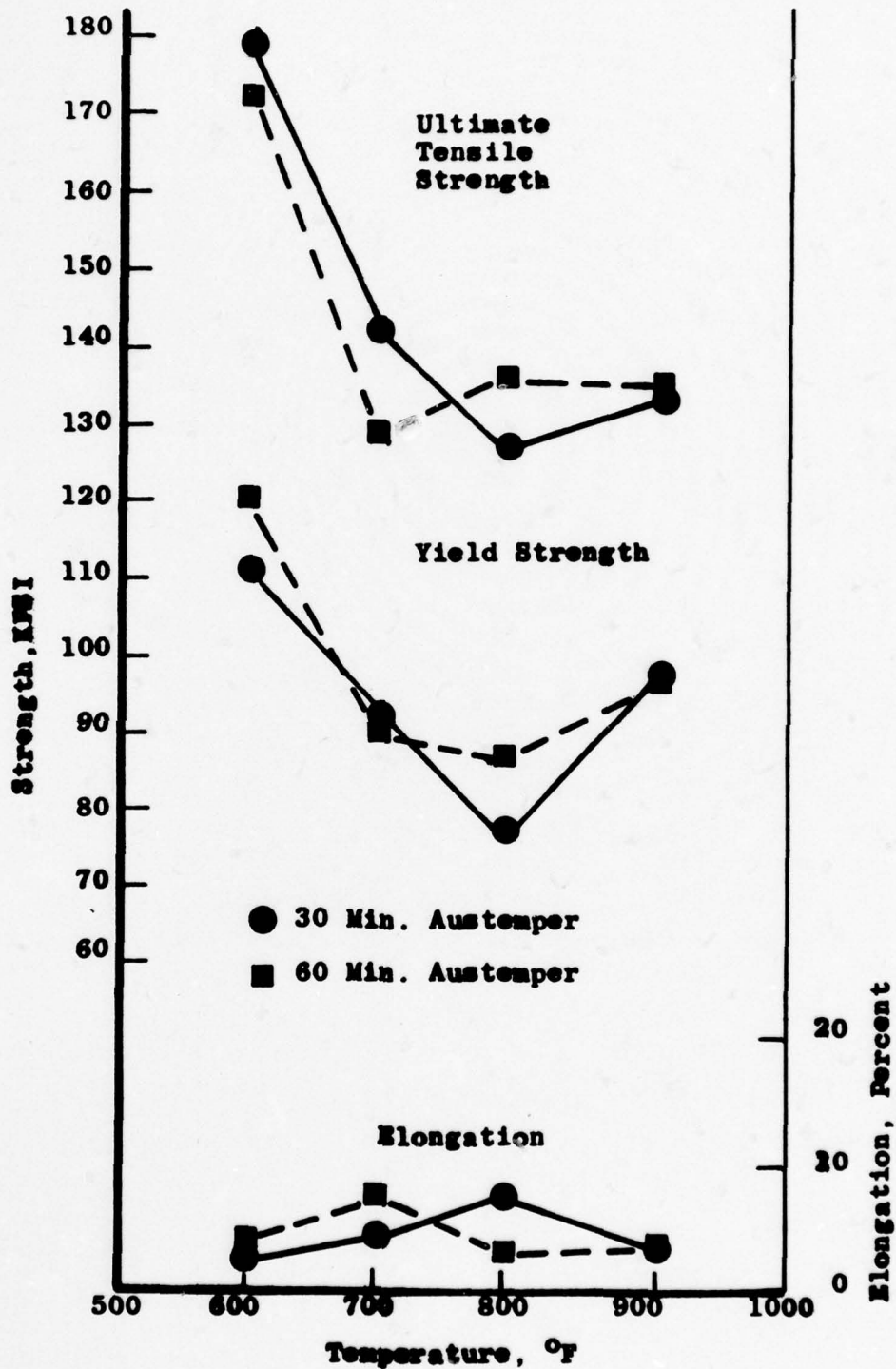
Mechanical Properties of a Ductile Iron Containing 1.5 Percent Nickel, Austempered at 1650°F and Austempered.
