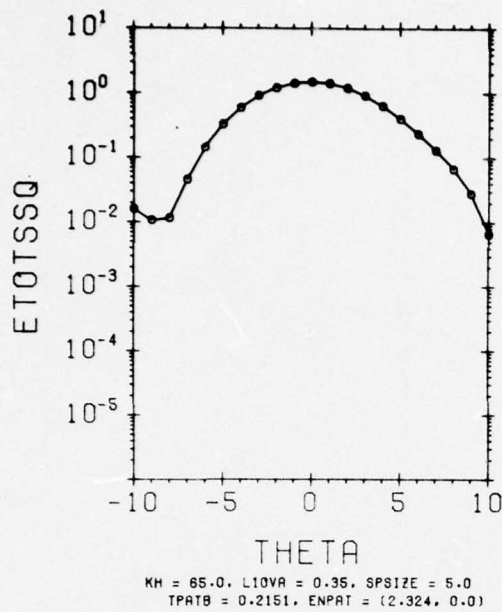
Figure 12. Sum Pattern of Rectangular Aperture (MIV), \text{ENPAT} = (2.324, 0.0) , \text{L1OVA} = 0.35
