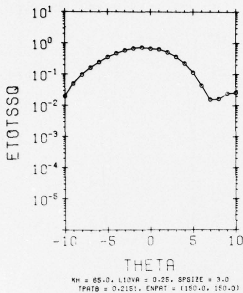
Figure 36. Sum Pattern of Rectangular Aperture (MIV), ENPAT = (150.0, 150.0), KH = 65.0, L10VA = 0.25
