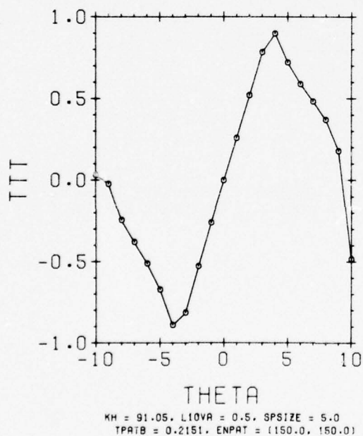
Figure 27. Sum Pattern of Rectangular Aperture (MIV), \text{ENPAT} = (150.0, 150.0) , \text{KH} = 91.05 , \text{L1OVA} = 0.5
