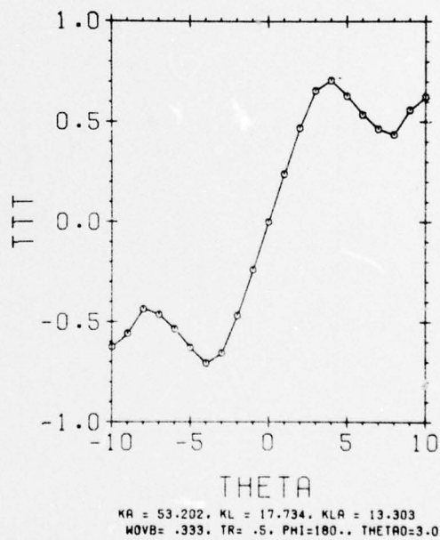
Figure 58. Tracking Signal (MV), \text{TR} = 0.5 , \text{PHI} = 180.0^\circ , K_{LA} = 13.303
