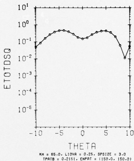
Figure 37. Difference Pattern of Rectangular Aperture (MIV), ENPAT = (150.0, 150.0), KH = 6.5, L10VA = 0.25
