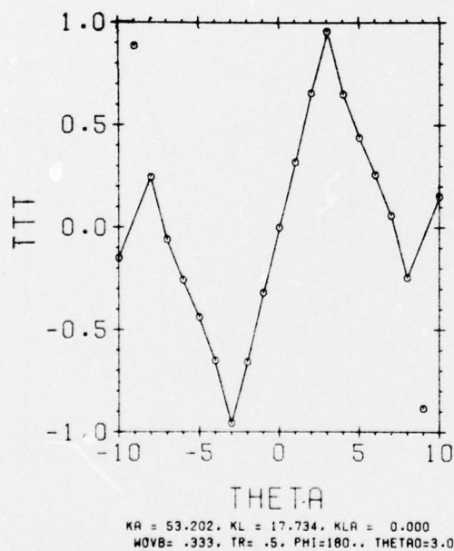
Figure 57. Tracking Signal (MV), \text{TR} = 0.5 , \text{PHI} = 180.0^\circ , K_{LA} = 0.0
