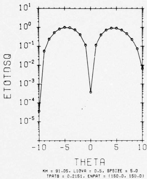
Figure 28. Difference Pattern of Rectangular Aperture (MIV), \text{ENPAT} = (150.0, 150.0) , \text{KH} = 91.05 , \text{L1OVA} = 0.5
