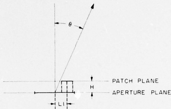
Figure 1. Simple Aperture Blocking Model Square Aperture
