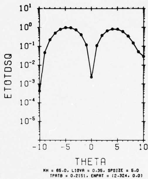
Figure 13. Difference Pattern of Rectangular Aperture (MIV), \text{ENPAT} = (2.324, 0.0) , \text{L1OVA} = 0.35
