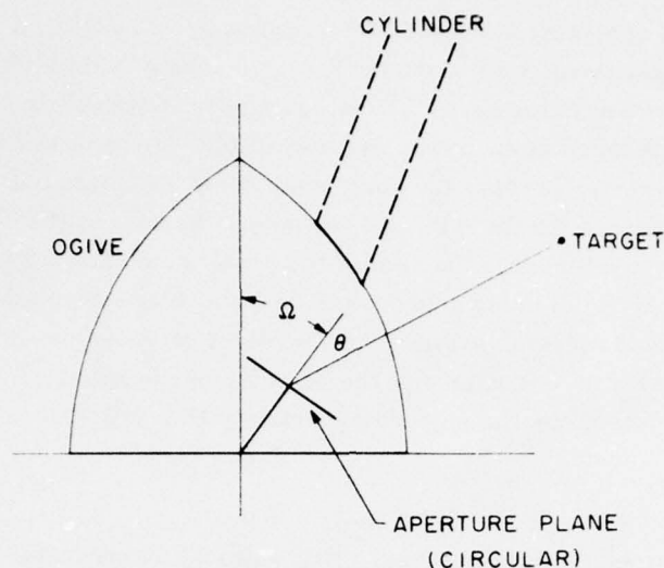
Figure 3. Ogival Radome, Plane-Wave Spectrum - Surface Integration Method
