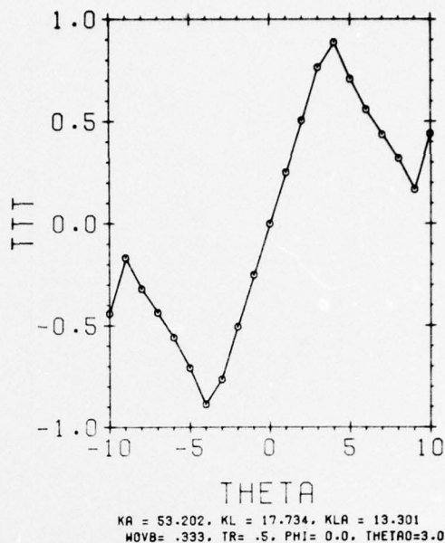
Figure 52. Tracking Signal (MV), TR = 0.5, PHI = 0.0° (no patch)
