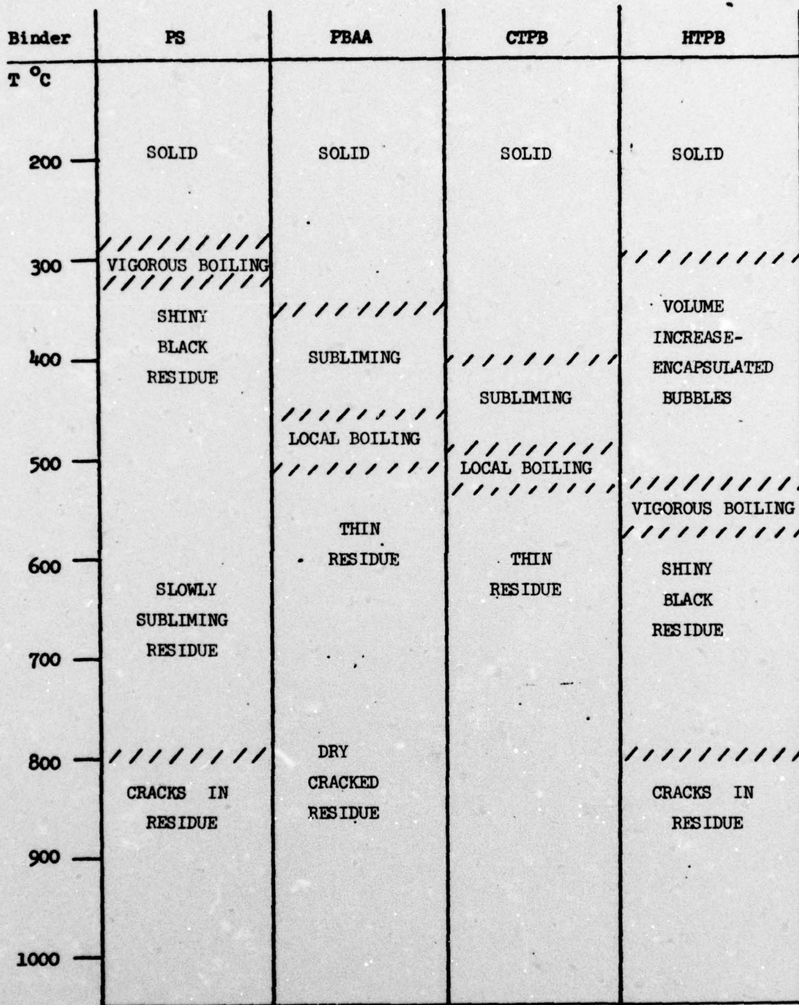
THERMAL DECOMPOSITION OF BINDERS IN AIR
