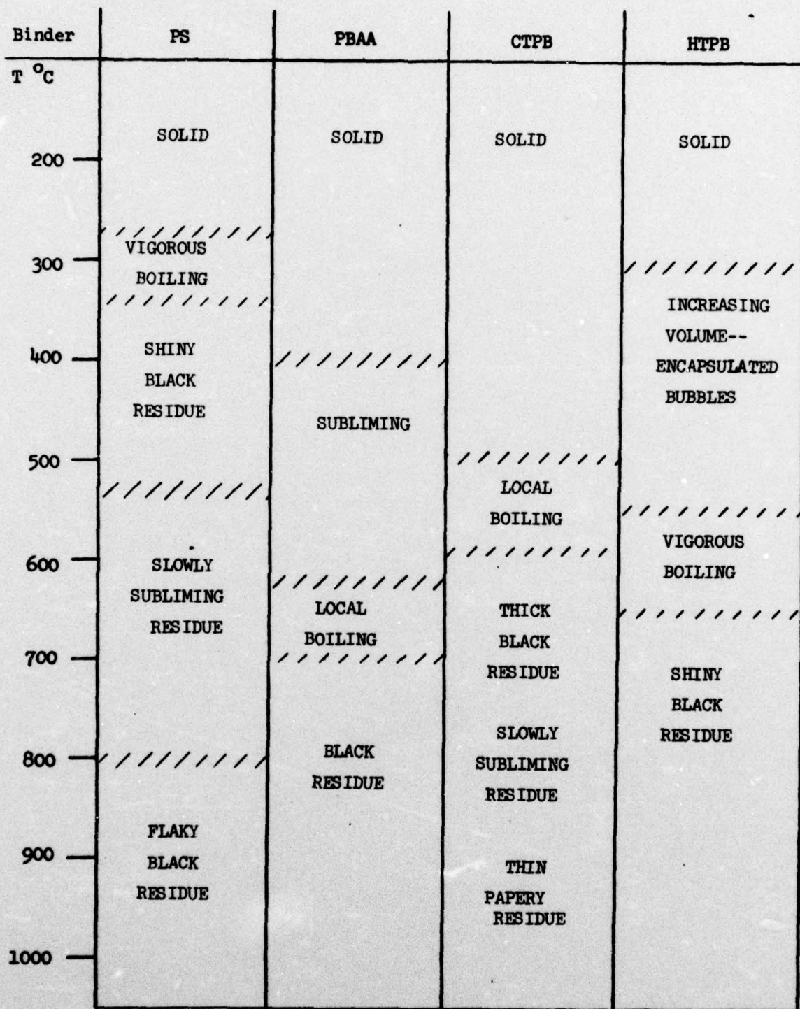
THERMAL DECOMPOSITION OF BINDERS IN ARGON
