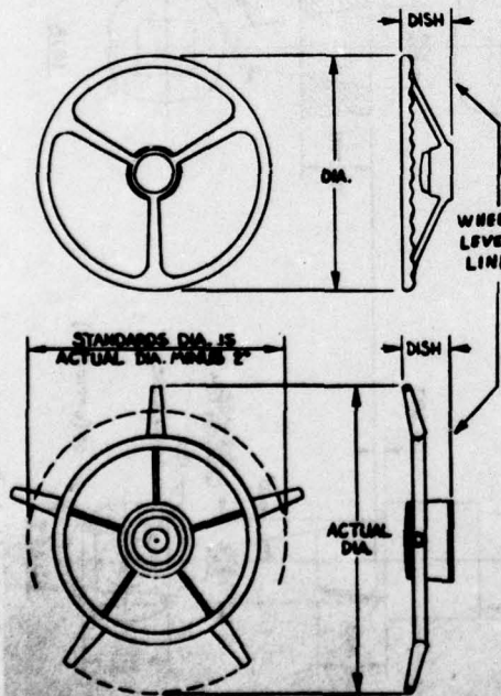
FIGURE 5 - WHEEL DESCRIPTION
