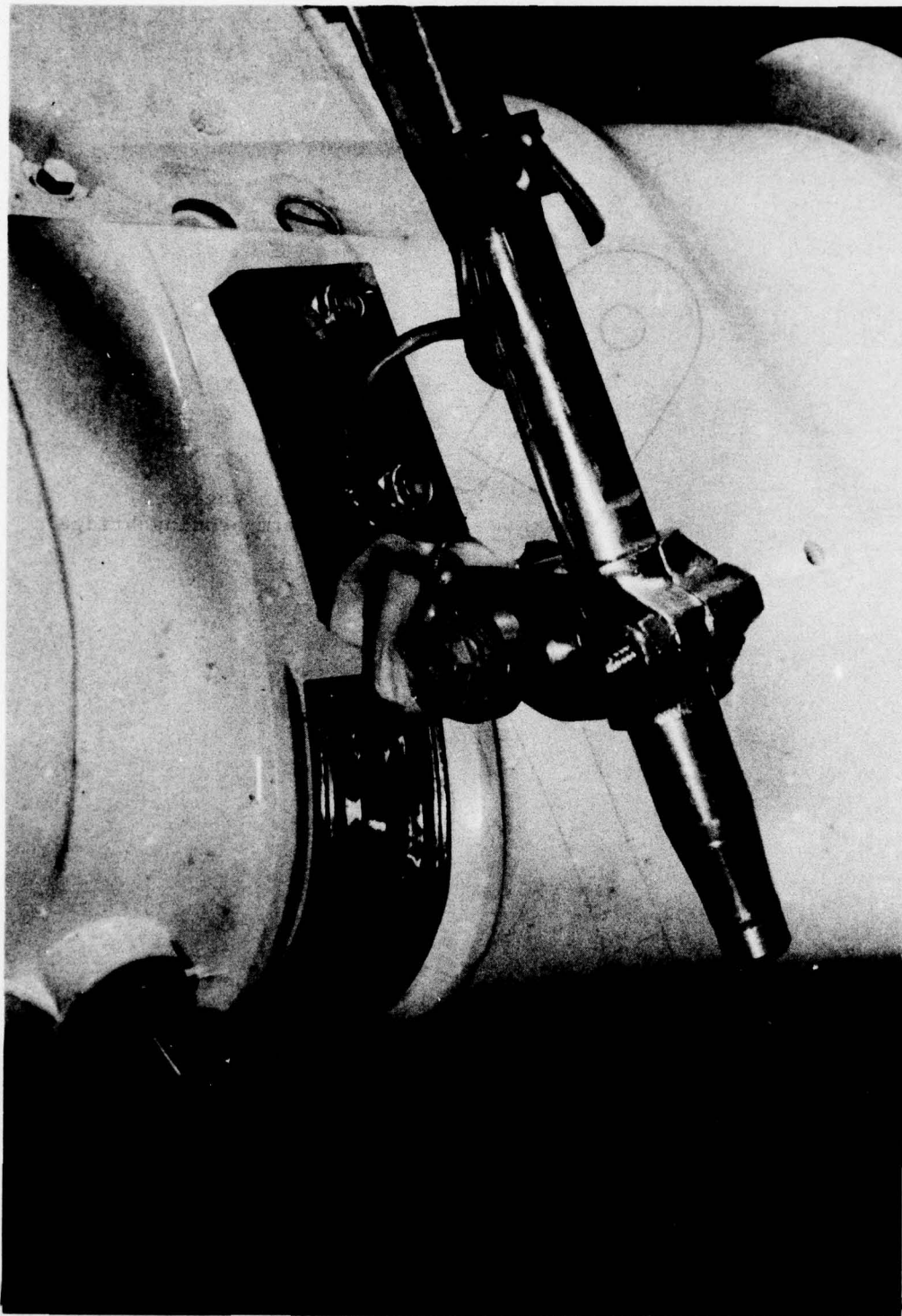
FIGURE 4. STERN DRIVE STEERING BRACKET.
