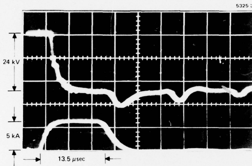
Figure 3. Fifty (50) pulse burst (at 60 Hz), 5 kA, 24 kV.
