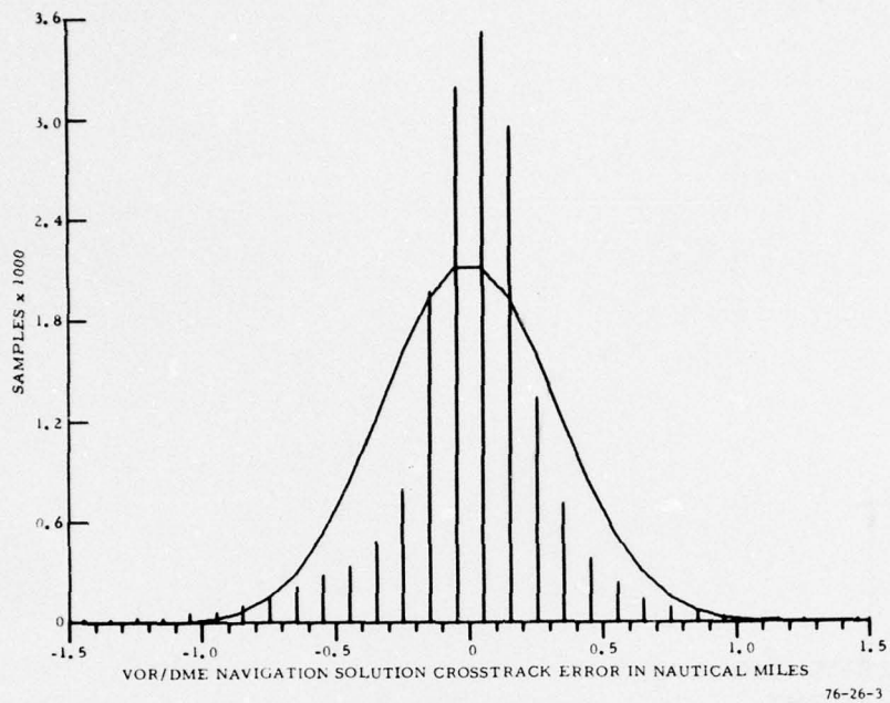
FIGURE 3. VOR/DME NAVIGATION SOLUTION CROSSTRACK ERROR DISTRIBUTION
