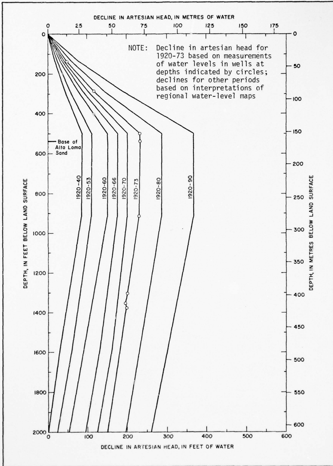
FIGURE 29-Approximate decline in artesian head
