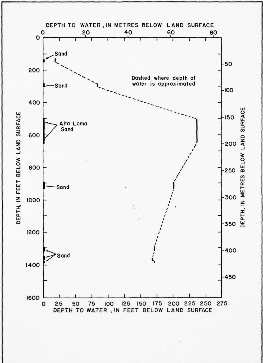
FIGURE 27.-Potentiometric profile at Seabrook, July 1974
