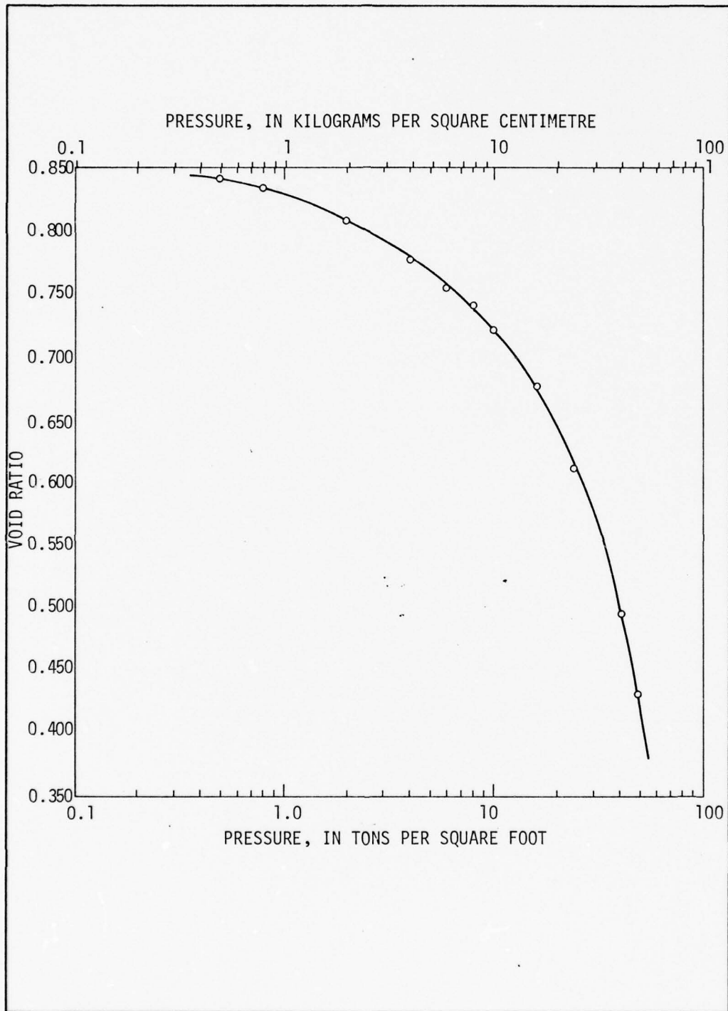
FIGURE 12.-Relation between void ratio and applied pressure for a clay sample from a depth of 221 feet (67 m), well LJ 65-32-503
