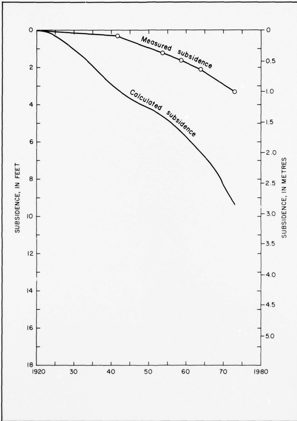
FIGURE 28.-Land-surface subsidence calculated on the basis of consolidation theory, 1920-73
