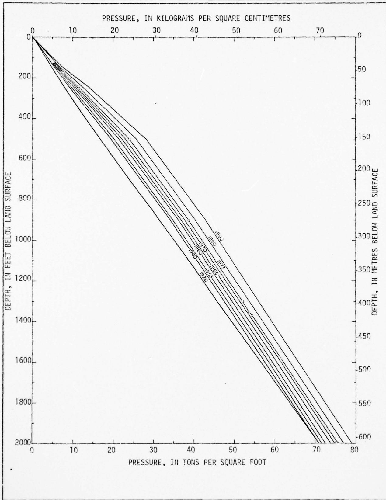
FIGURE 26. Effective load at Seabrook for depths between 0 and 2000 feet (0 and 610 m)
