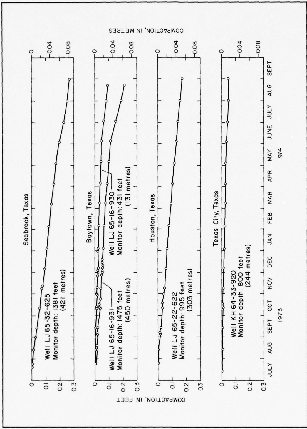
FIGURE 8.-Measured compaction in the Houston-Galveston region, July 1973-August 1974
