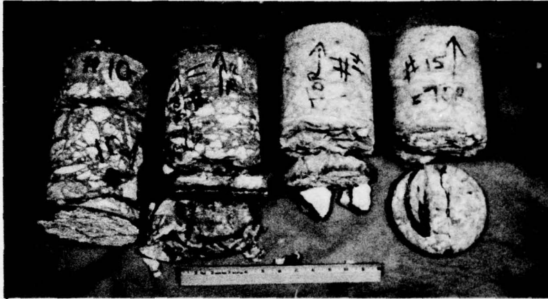
b. North span (cores 10, 11, 14, and 15)
