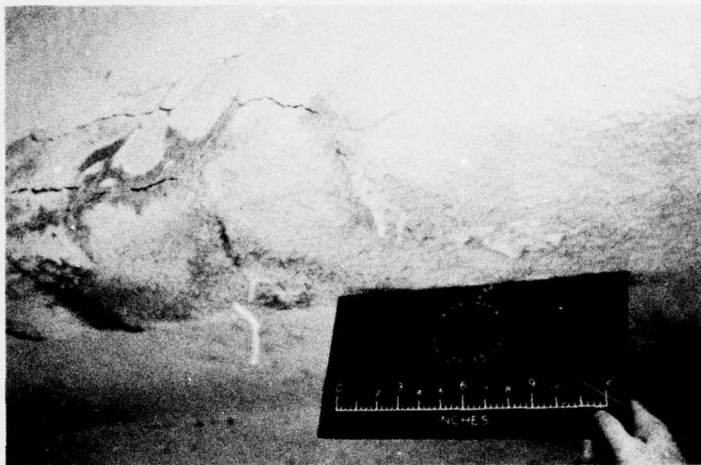
Figure 7. Leaching of floor beam
