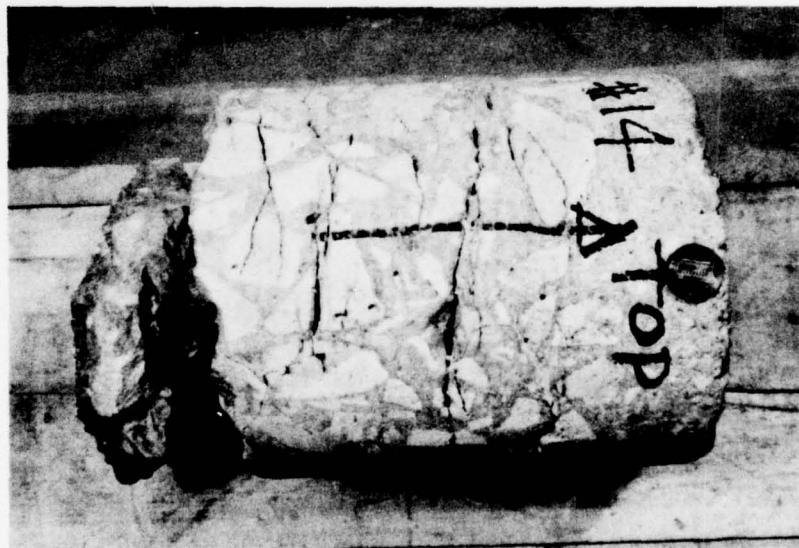
Figure 14. Concrete cores drilled from bridge deck
