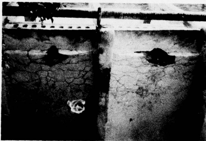
Figure 9. Underside of bridge deck
