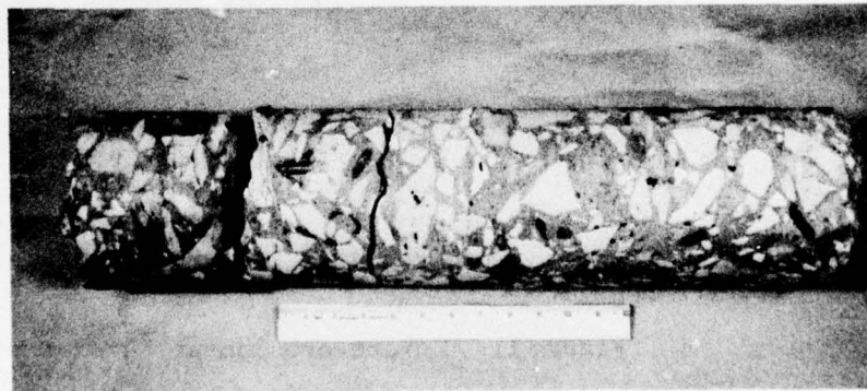
Figure 12. Concrete cores drilled from abutment
