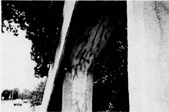
a. Cracks running parallel with arch
