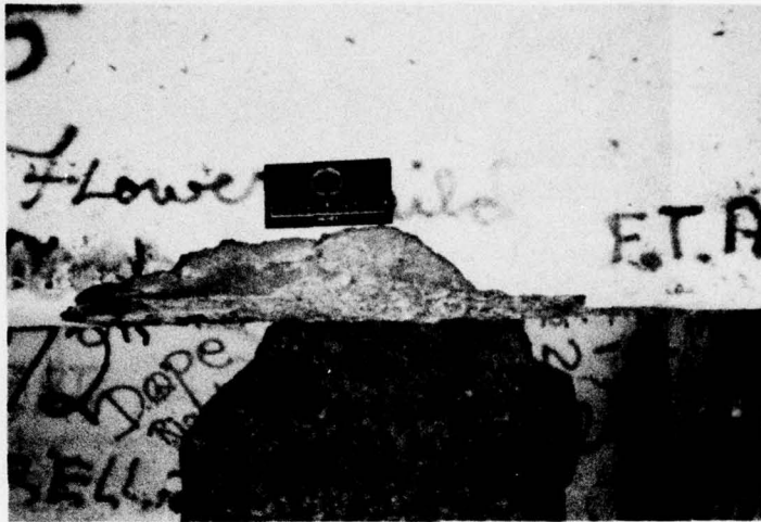
Figure 10. Large spalling of shotcrete surface of abutment
