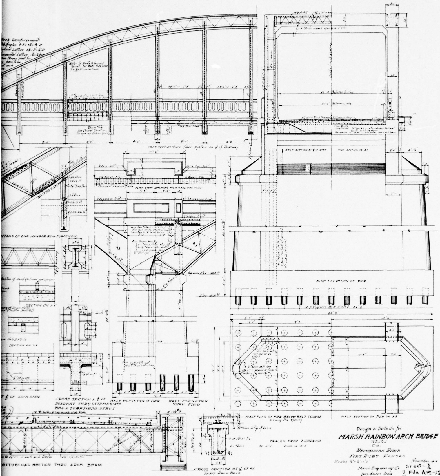
Figure 2. Design details for Marsh Arch Bridge
