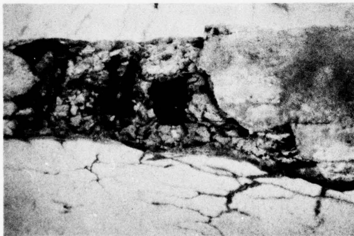
Figure 6. Floor beams showing spalling and cracking
