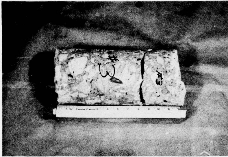
Figure 13. Concrete core drilled from arch rib (south end, downstream)
