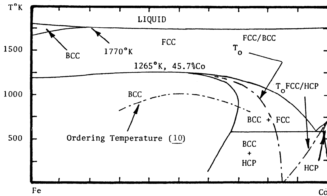
Figure 3. Calculated Iron-Cobalt Phase Diagram Showing Locus of Curve for T_o(\text{FCC/BCC}) where FCC and BCC Phases of Same Composition Have Equal Free Energies (9,10).
