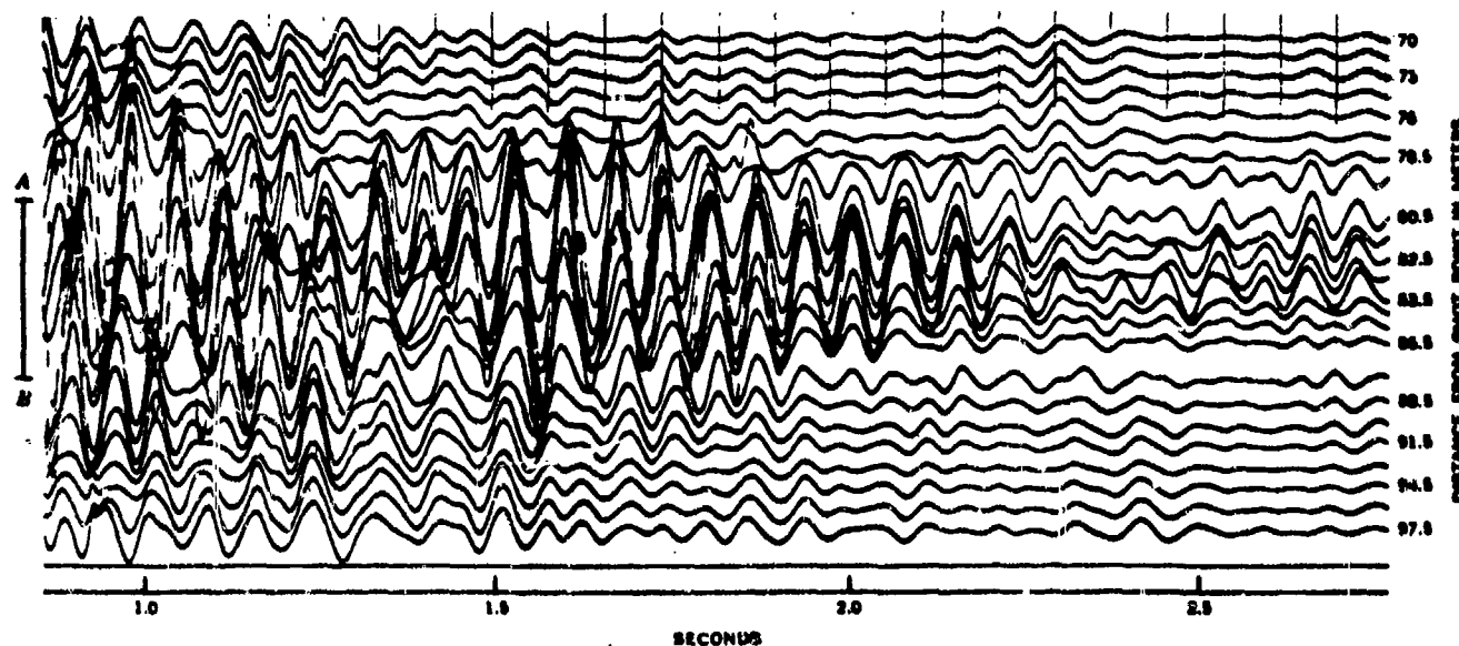
FIGURE 1.—Part of a seismogram recorded over a lava tunnel in the Pisgab lava flow, San Bernardino County, Calif. Note prominent in-phase cavity oscillations in center of seismogram. AB indicates the location and approximate width of the tunnel.
