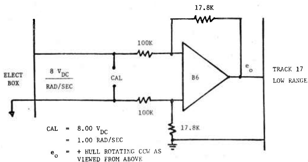
TRACK 17 HULL YAW VELOCITY
