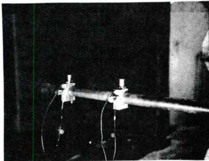
Figure 62 Mounted Accelerometers for Barrel Whip Test
