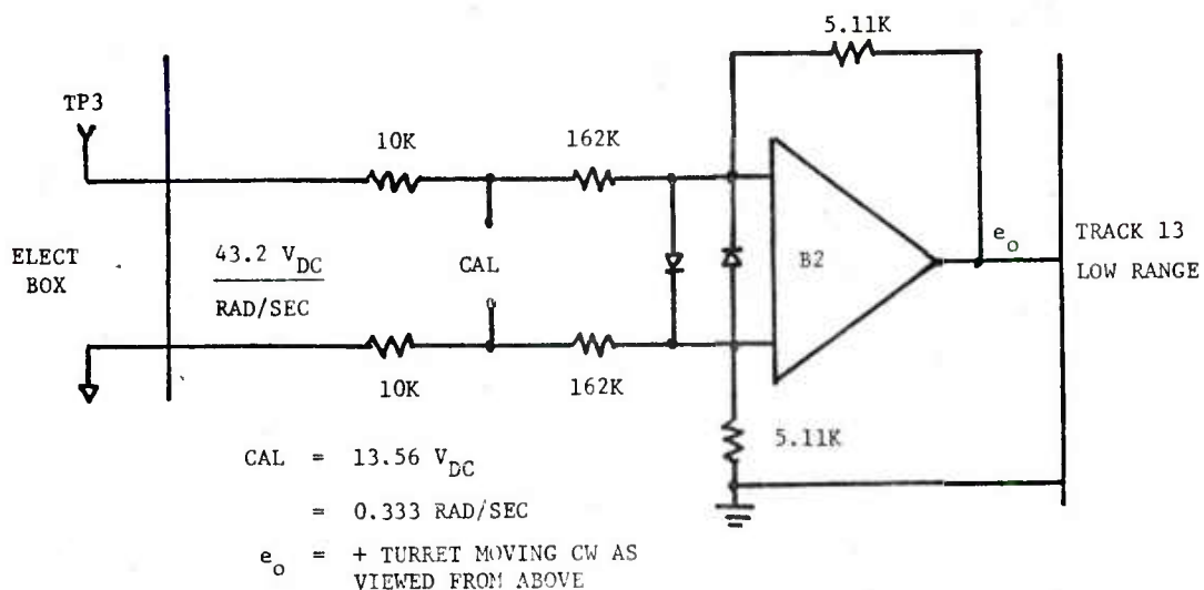
TRACK 13 GUN TRAVERSE VELOCITY
