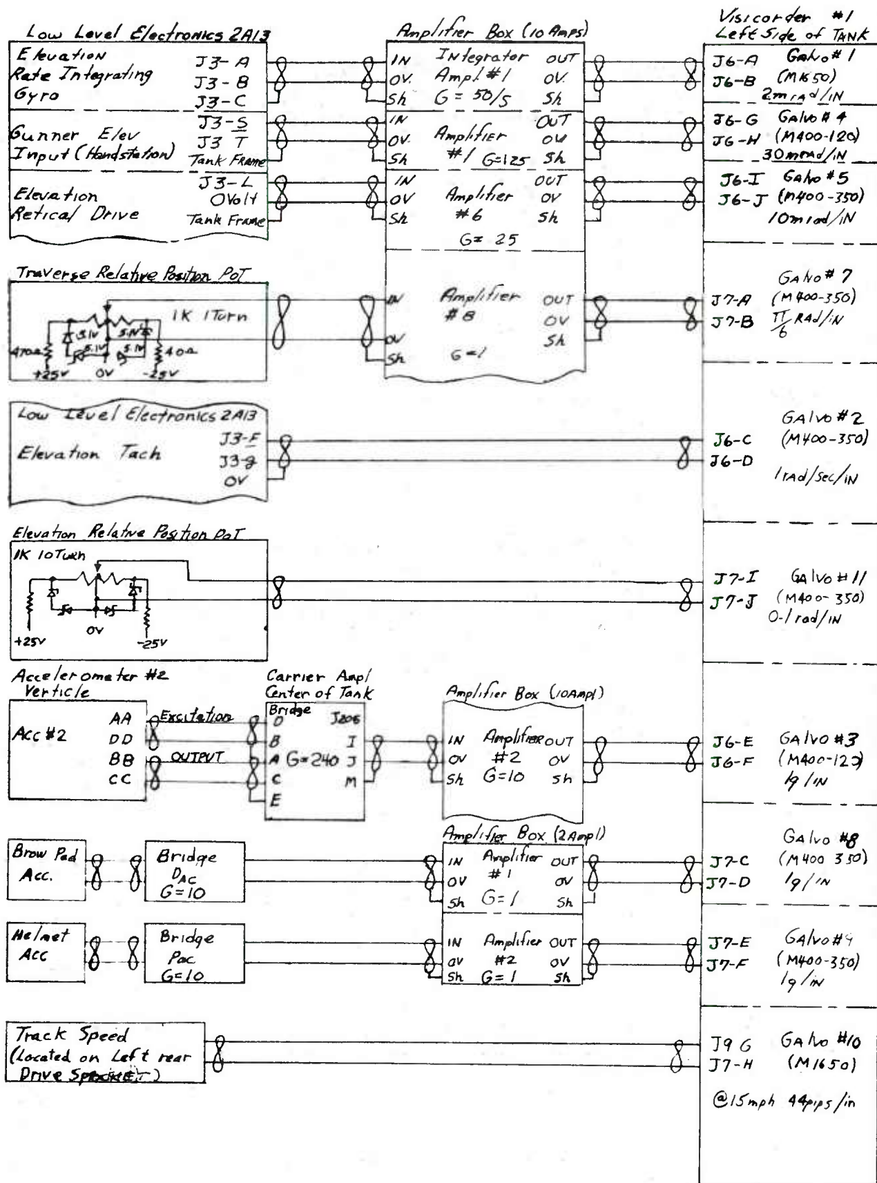
Figure 13 Instrumentation Schematic (Visicorder #1)
