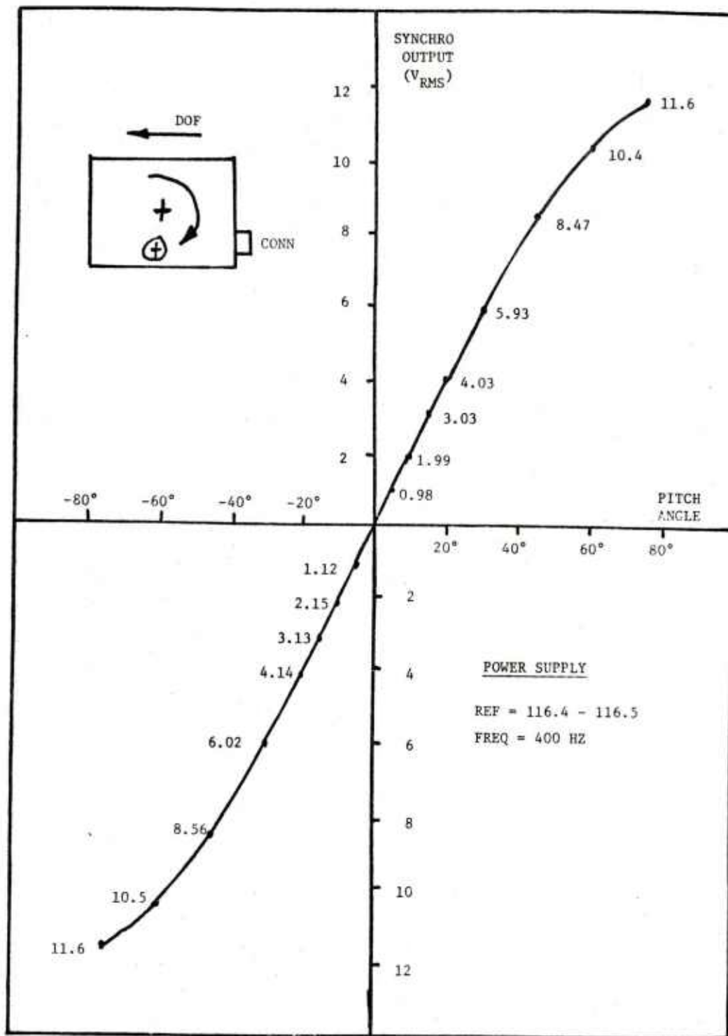
Figure 40 Vertical Gyro Calibration (Gyro Pitch Axis) for Track 19
