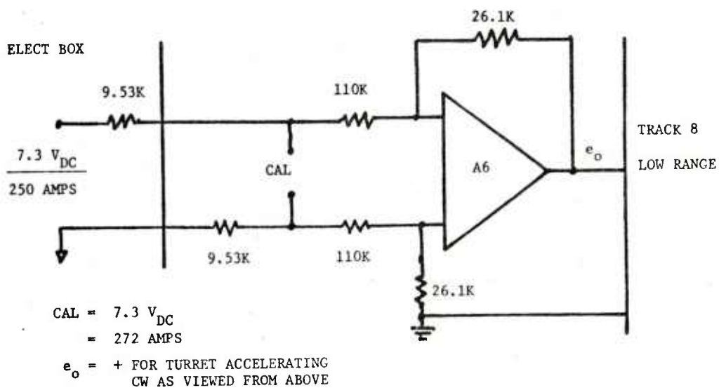
TRACK 8 TRAVERSE MOTOR CURRENT
