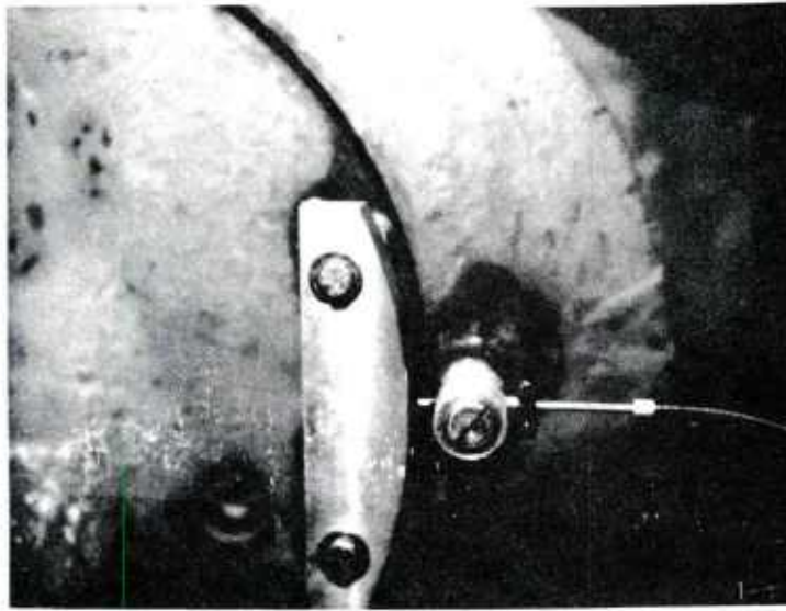
Figure 58 Fotonic Sensor Sensing Right End Shield Motion
