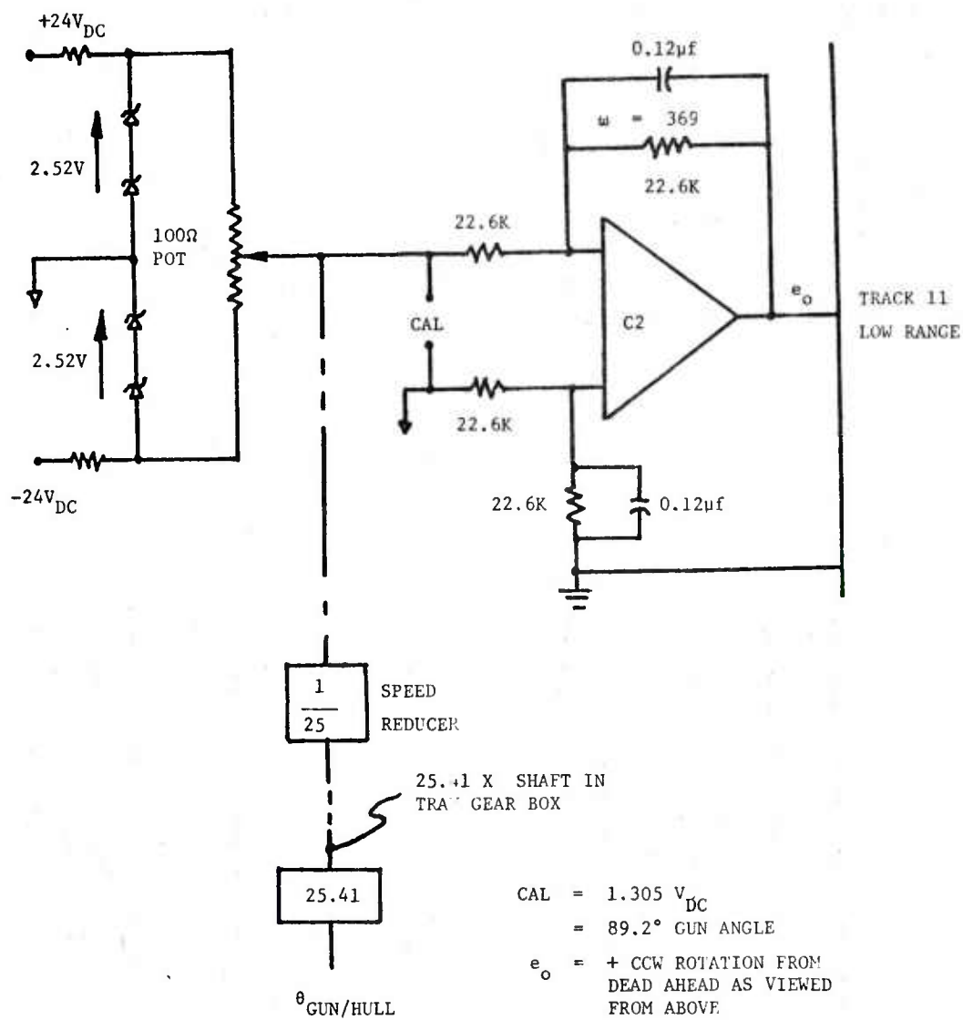
TRACK II GUN TRAVERSE POSITION
