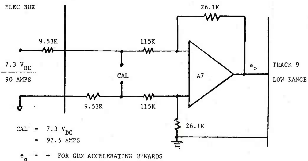
TRACK 9 ELEVATION MOTOR CURRENT
