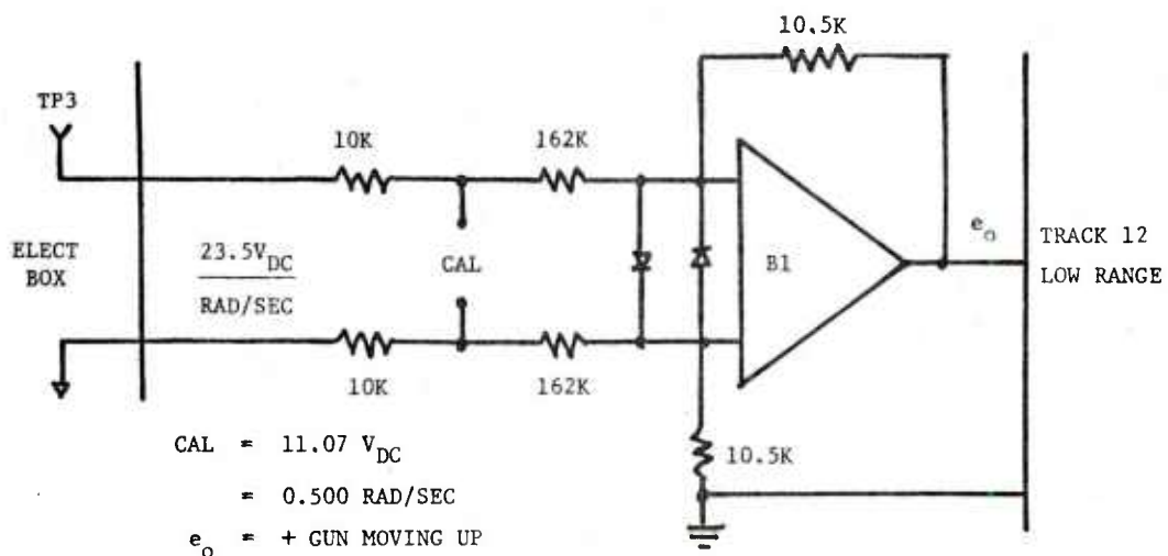
TRACK 12 GUN ELEVATION VELOCITY
