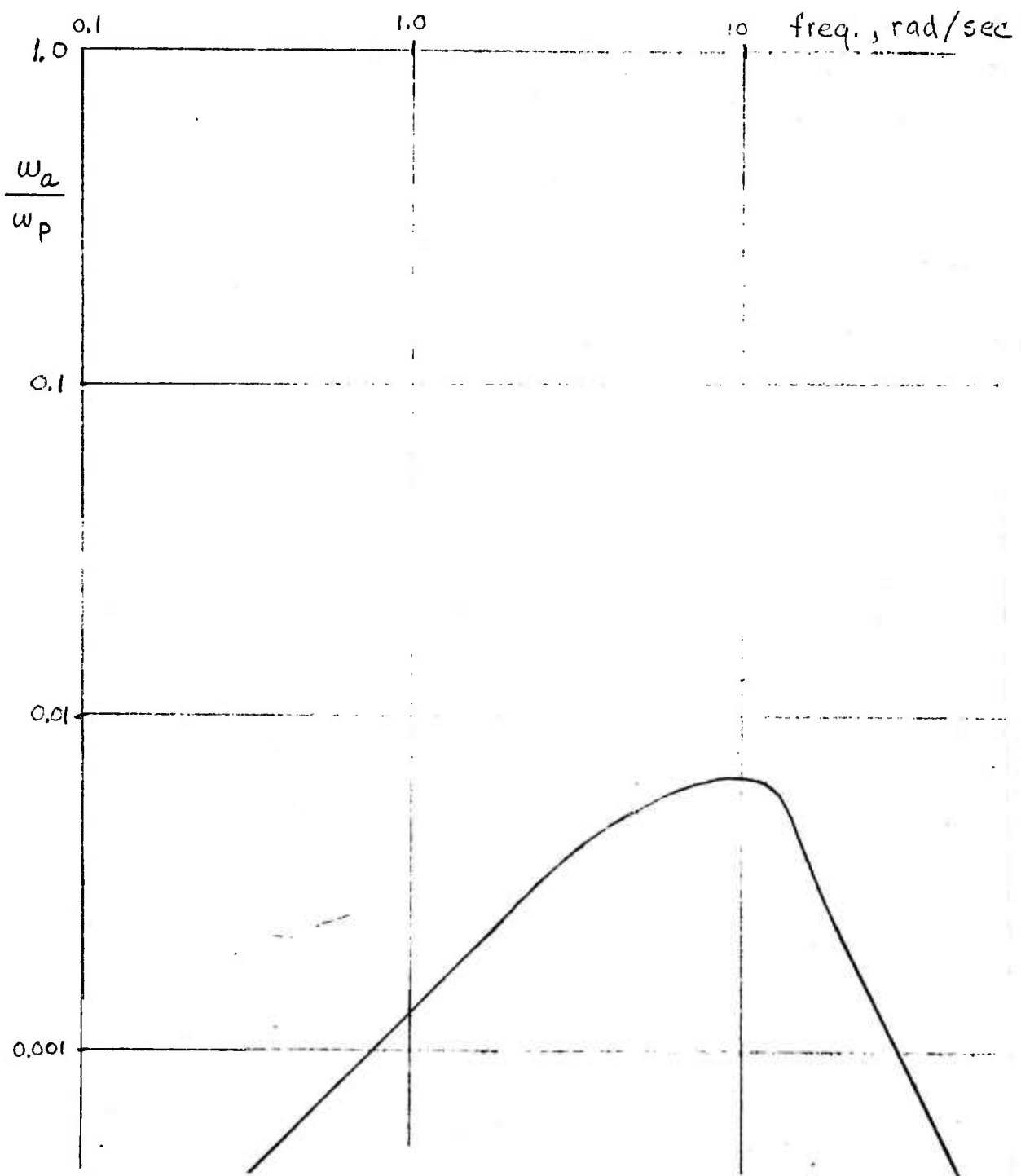
Figure 95 Sensitivity of Tracking Rate - Measurement to Pitch Rate 6-10
