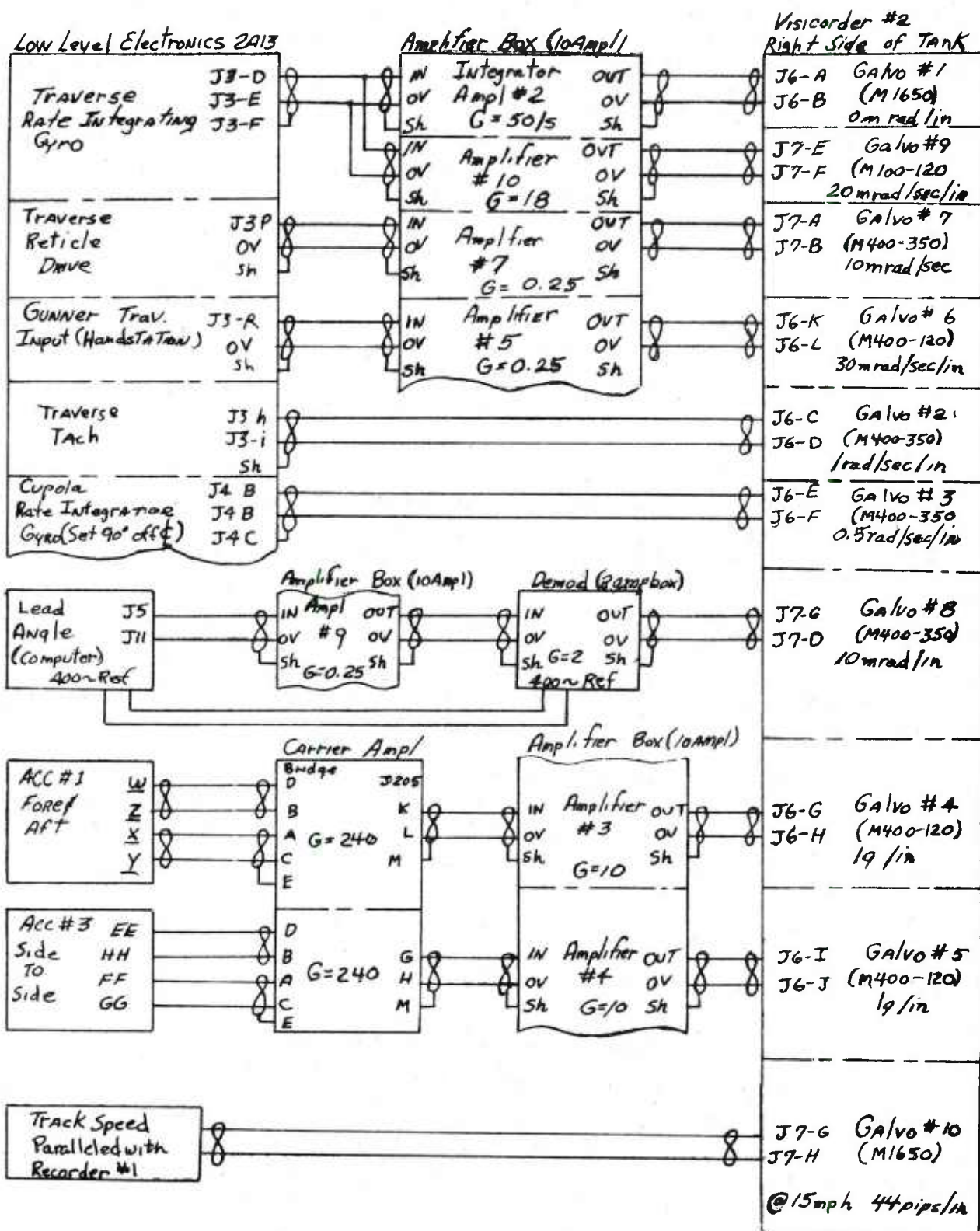
Figure 14 Instrumentation Schematic (Visicorder #2)
