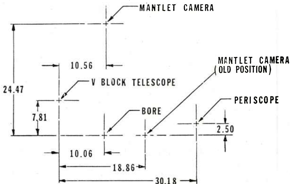
Figure 2 Instrumentation Alignment (All Dimensions in Inches)
