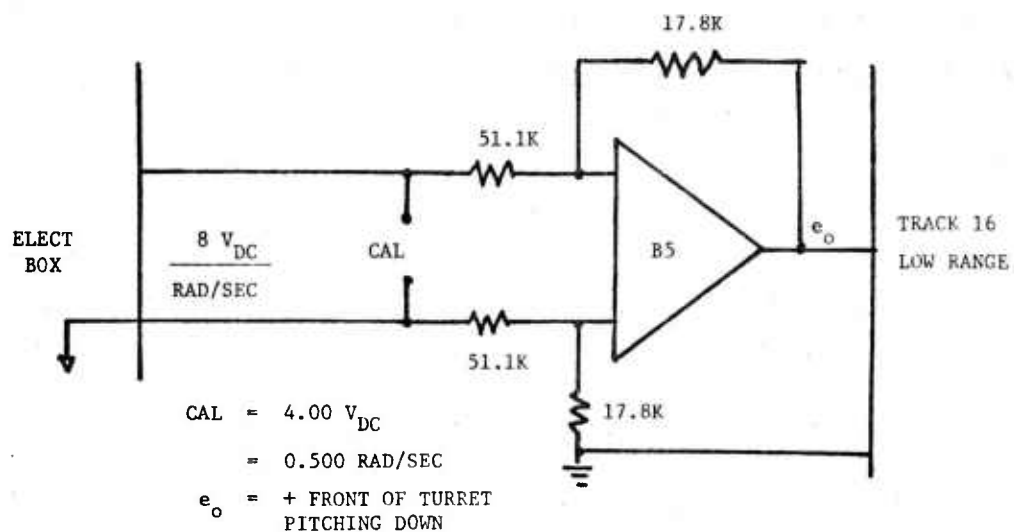
TRACK 16 TURRET PITCH VELOCITY
