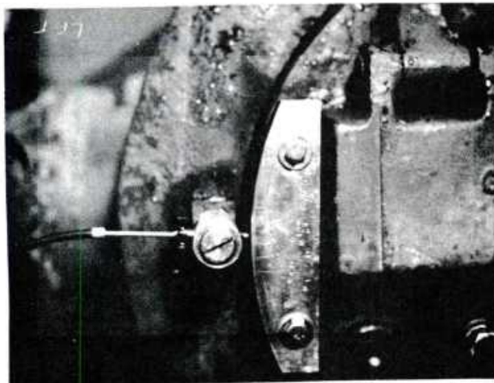
Figure 59 Fotonic Sensor Sensing Left End Shield Motion
