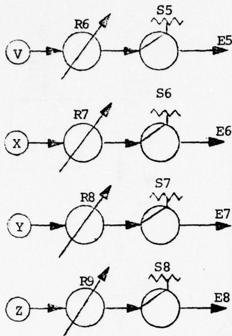
Figure 66: N1-Nonlinearity #1 Schematic Diagram (2 of 3).
