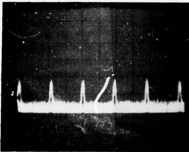
Figure 50: Detected radar signal. Pulsed NOISE only. (Signal parameters: PRF = 1 KHZ, PW = 100 \mu\text{s} , NOISE attenuator = 0 dB. Measured at "TEST OUT" in C1. E5 attenuator at 0 dB.)
