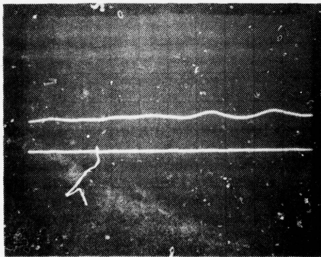
Figure 59: Power spectrum density of E10-GAUSSIAN NOISE. (Noise attenuator at 0 dB. Measured at "OUTPUT" in C1. Lower trace = spectrum analyzer noise level. Upper trace = E10 power spectrum density.)
