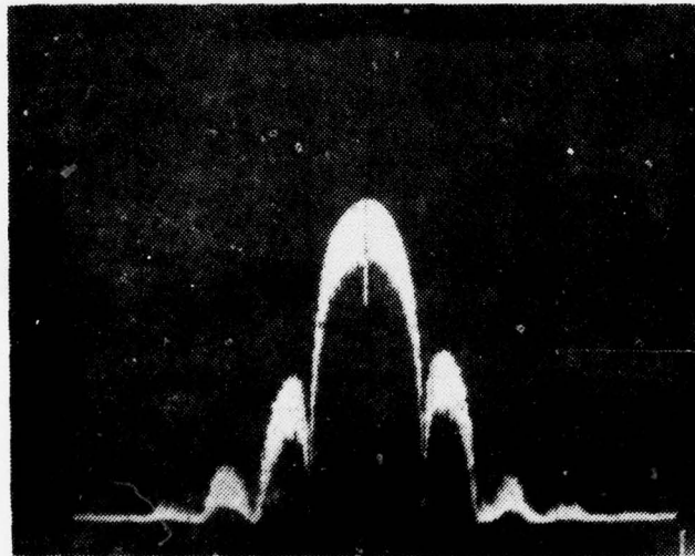
Figure 37: Frequency-domain view of E1. (Signal parameters same as in Figure 36. Measured at "TEST OUT" in C1.)
