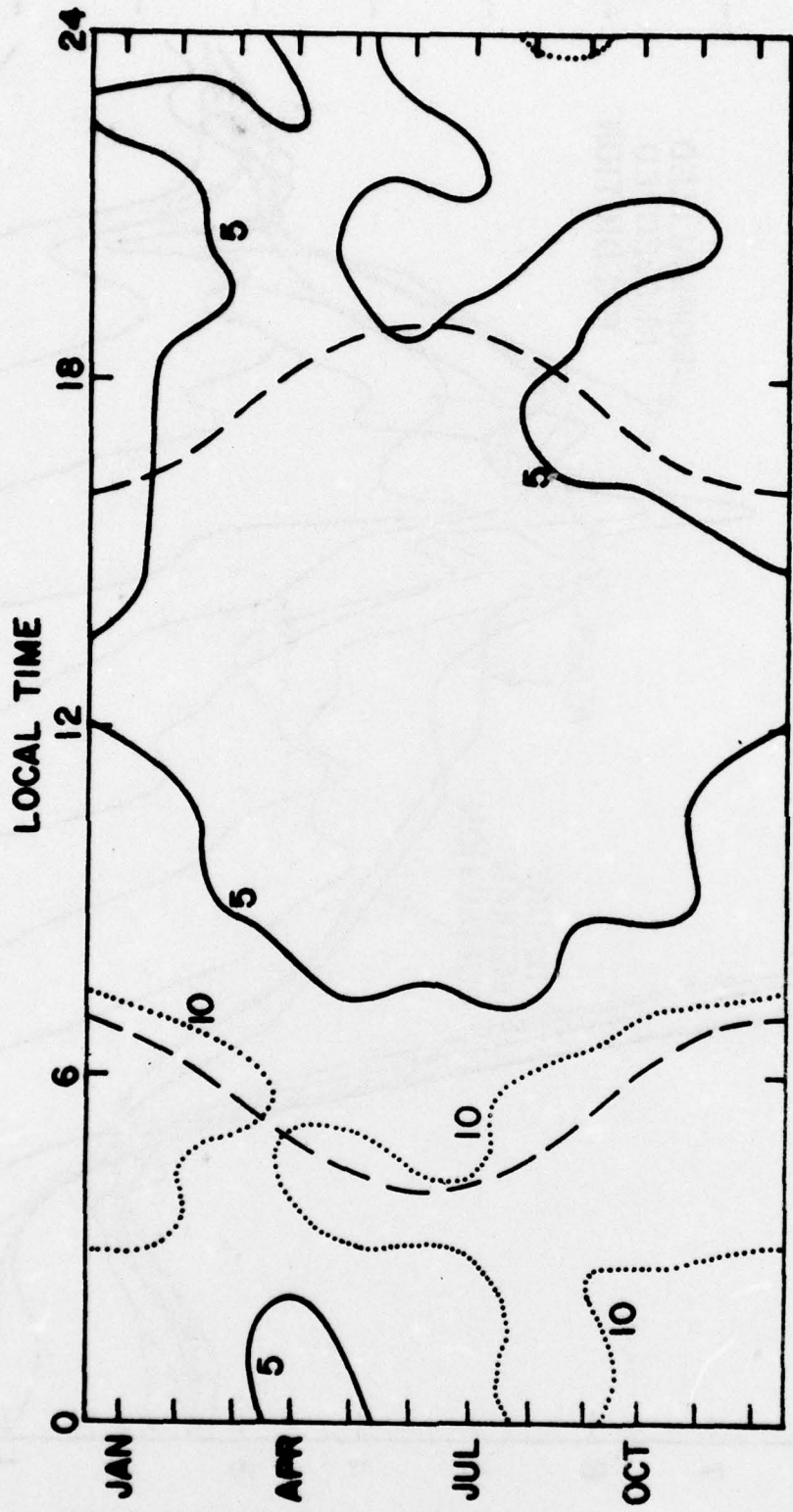
Figure 5 30-MINUTE PREDICTION
