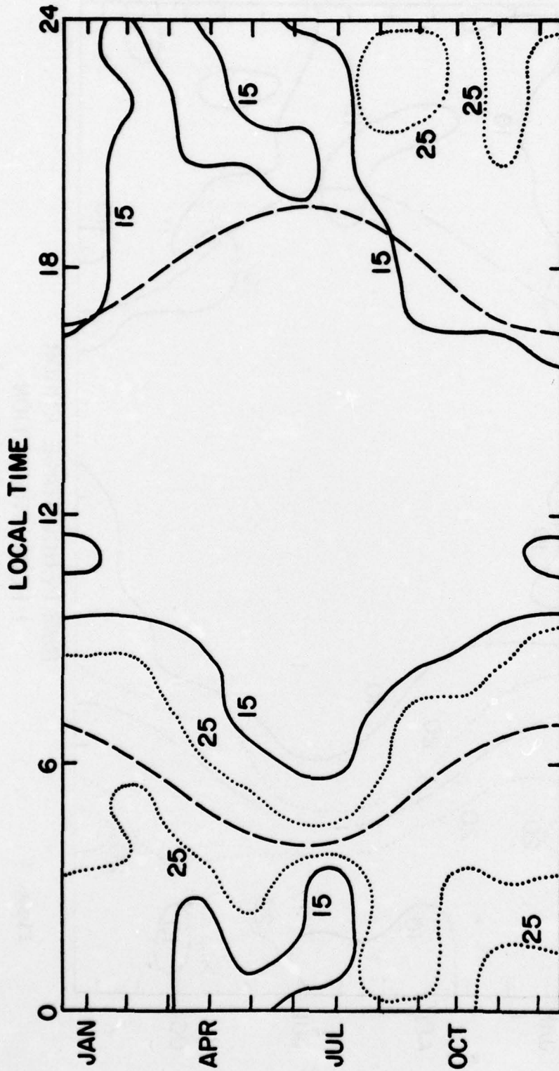
Figure 7 2-HOUR PREDICTION
