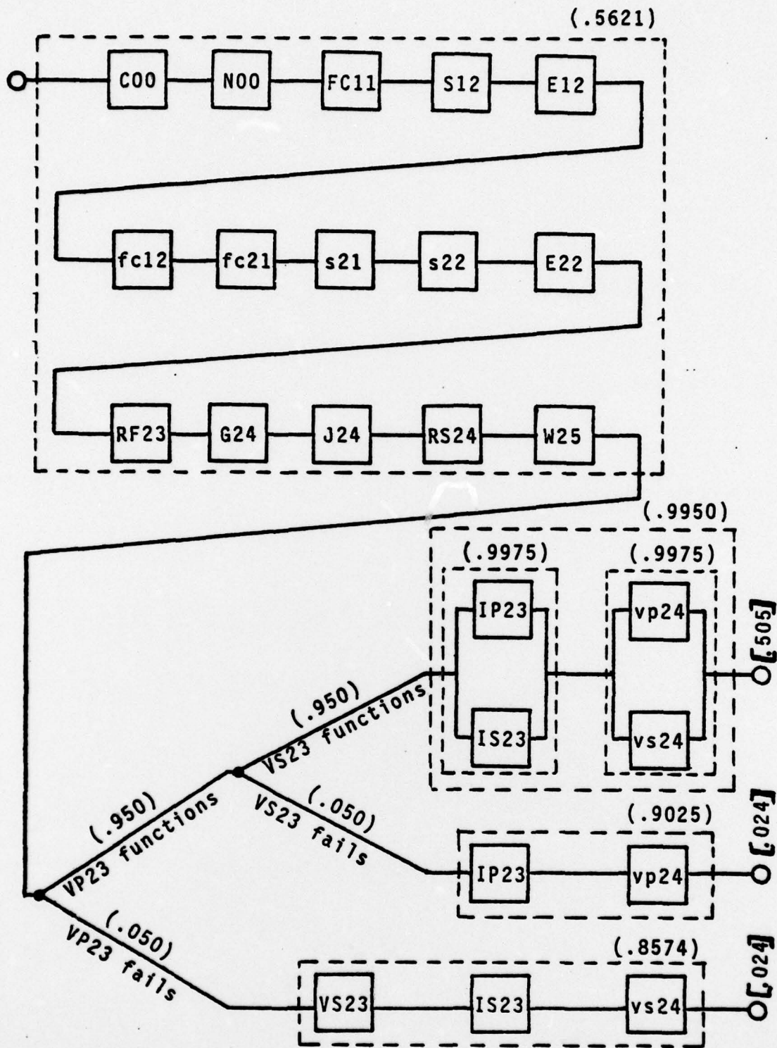
Figure 12 - REDUCTION INTO MODULES
