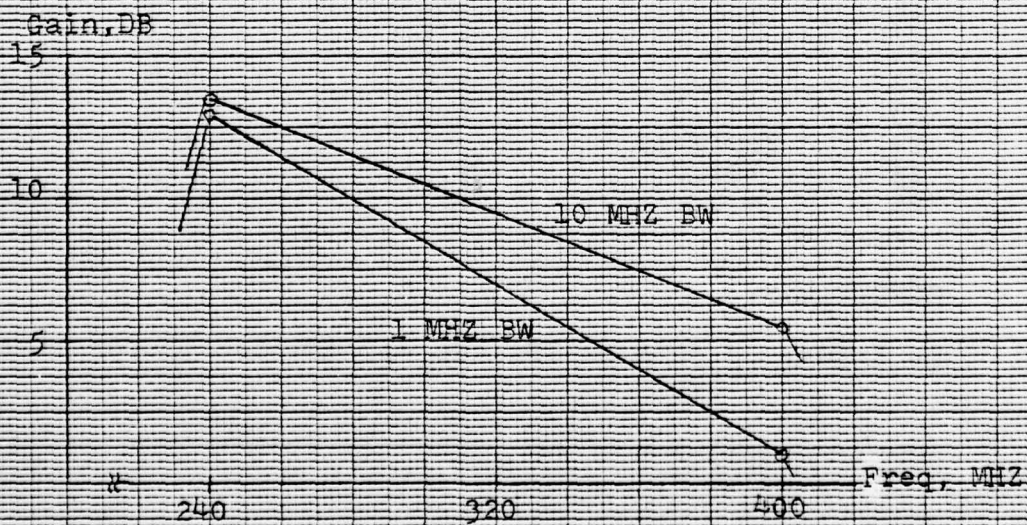
Figure 8.2. RF Channel Gain at TP22 vs. Frequency
