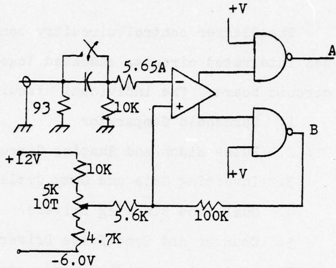
Figure 4.1. Threshold Comparator
