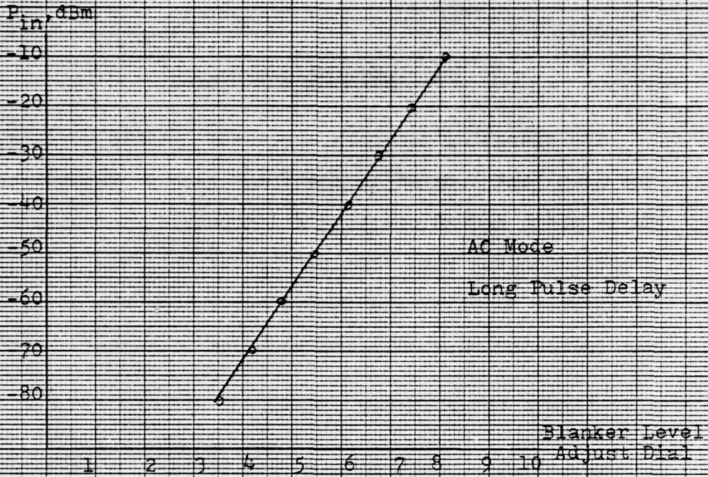
Figure 9.1.a. P_{in} vs. Dial Setting in 1 MHz BW
