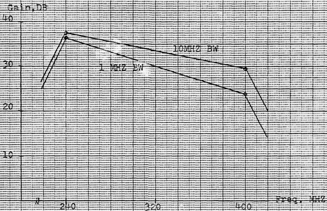
Figure 8.1. RF Channel Gain at TP26 vs. Frequency
