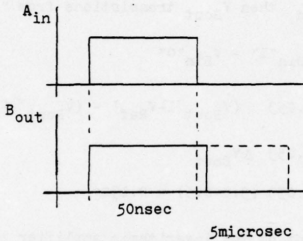
Figure 4.5. Pulse Width and Shaping Circuit
