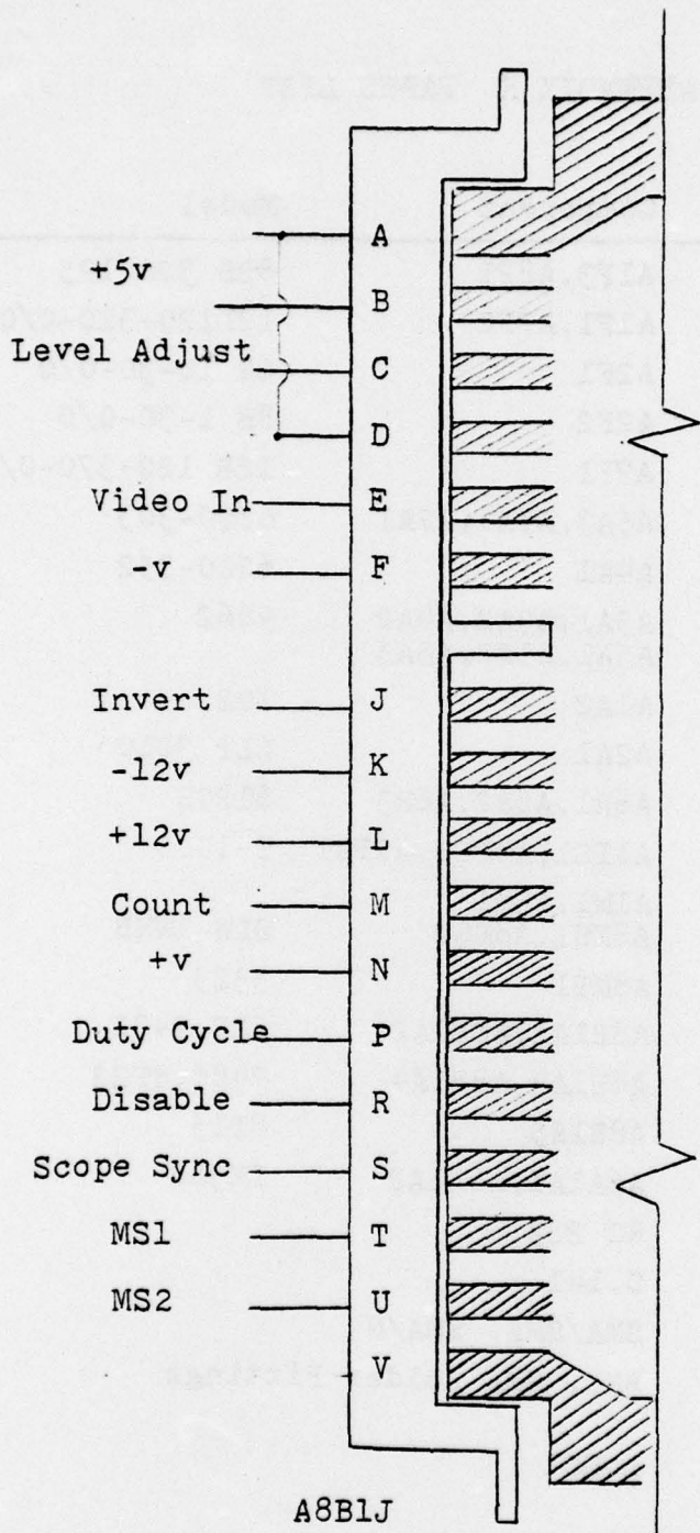
Figure G.5. Blanker Box Internal Wiring Connections
