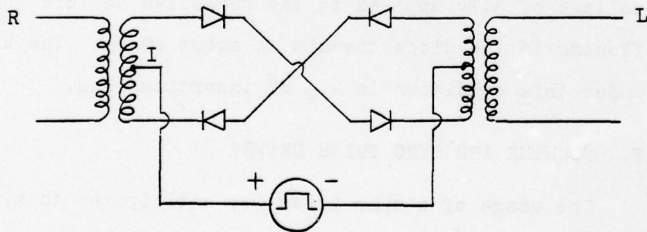
Figure 4.10. Blanker Switch
