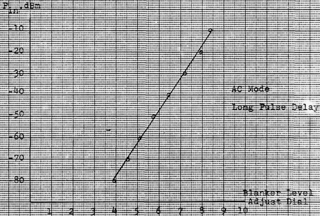
Figure 9.1.b. P_{in} vs. Dial Setting in 10 MHz BW
