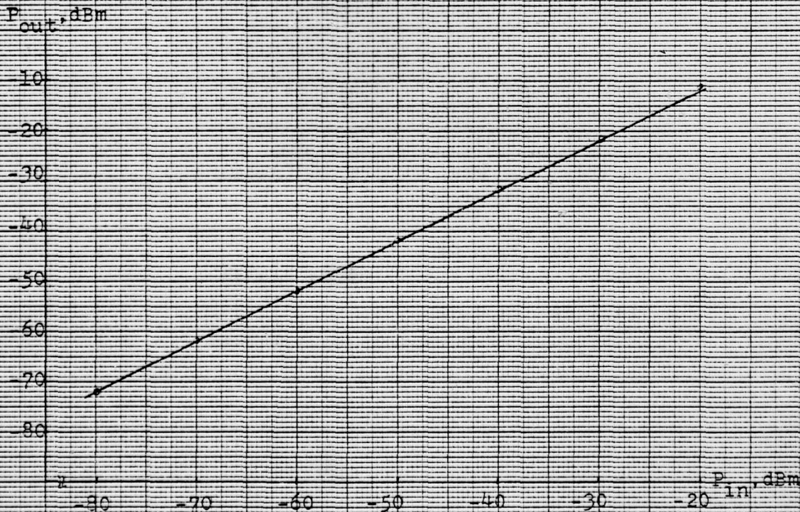
Figure 8.4. Blanker Channel Power Gain
