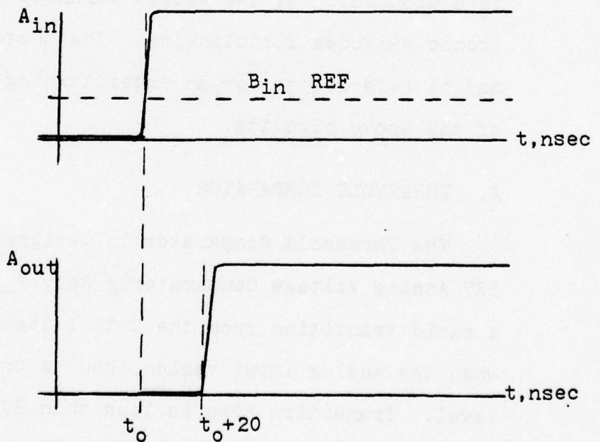
Figure 4.2. Comparator Waveforms
