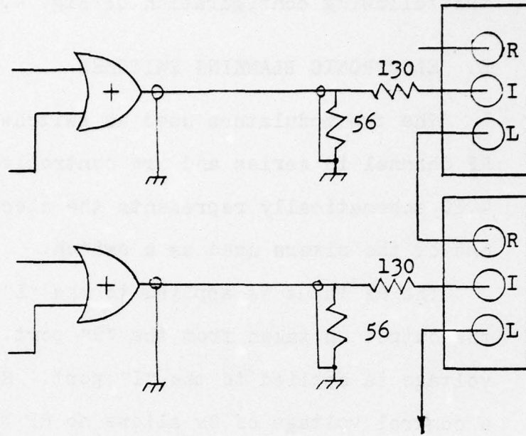
Figure 4.9. Blanker Switch--Driver Interconnections
