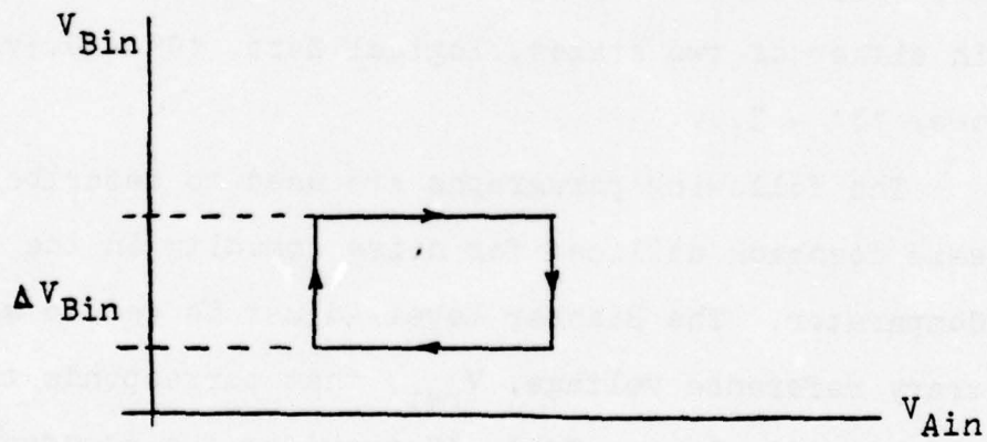
Figure 4.4. Hysteresis Loop
