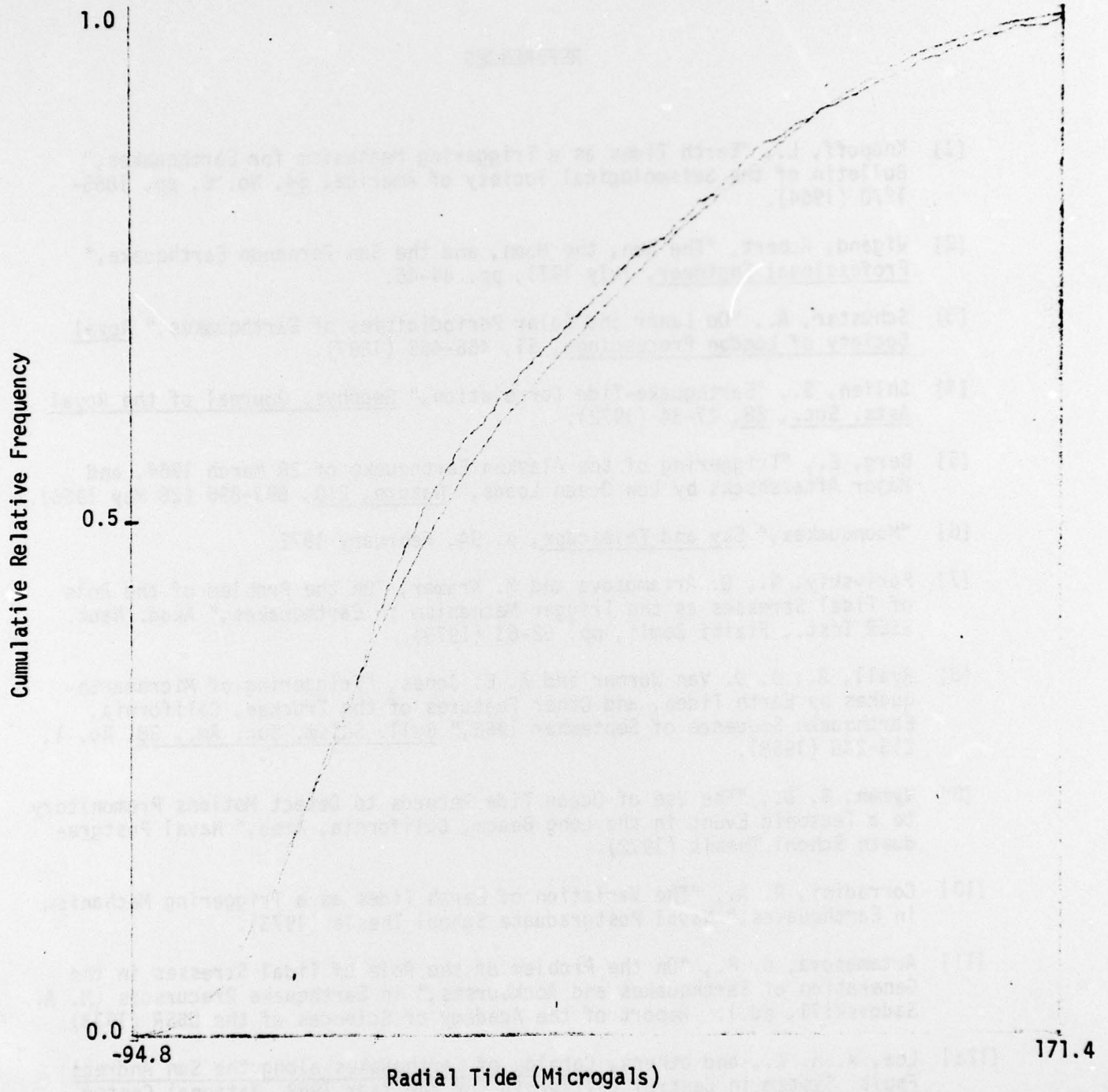
Figure 1. Plots of radial tide SCDF's for the sample of actual events and the simulated sample. The curve corresponding to the simulated sample is smoother than the other, due to the larger sample size involved.
