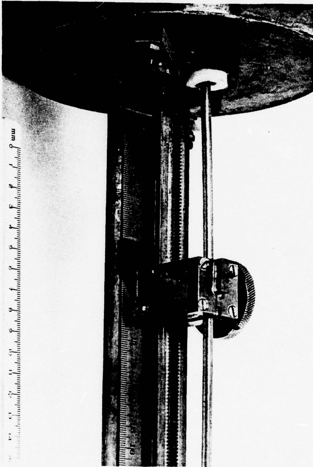
Figure 13. - Rack and pinion probe positioning mechanism
