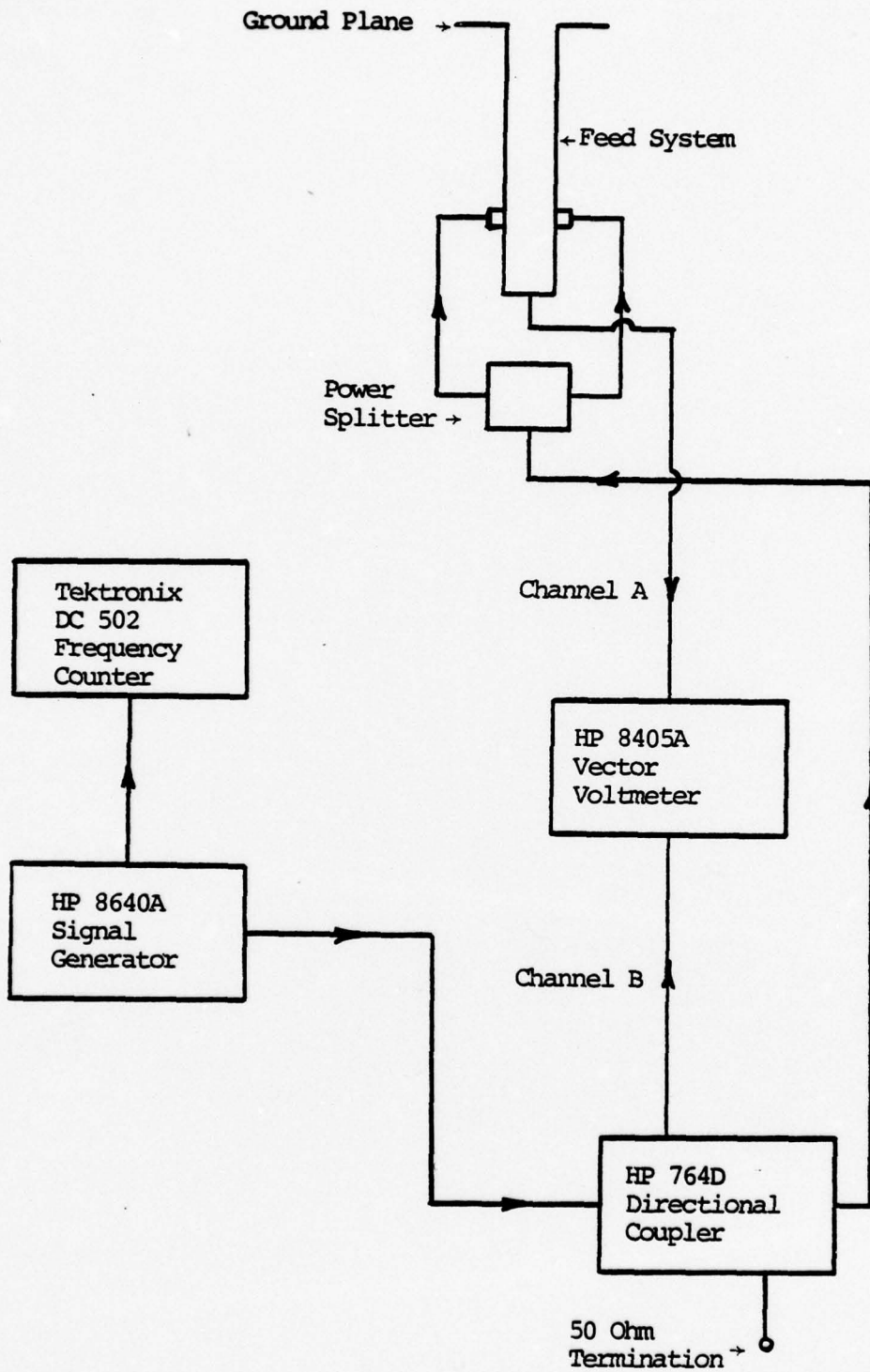
Figure 12. - Block diagram of instrumentation
