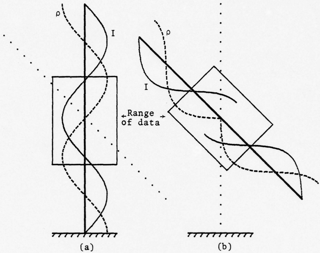
Figure 20. - Assumed charge and current density distributions for Case 2 crossed-monopole
