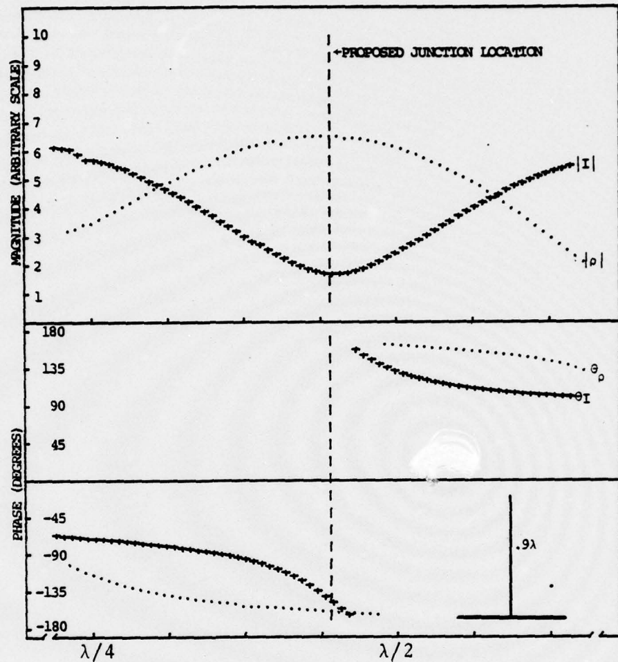
Figure 14. - Measured charge and current density distributions on the reference monopole at 195 Mhz
