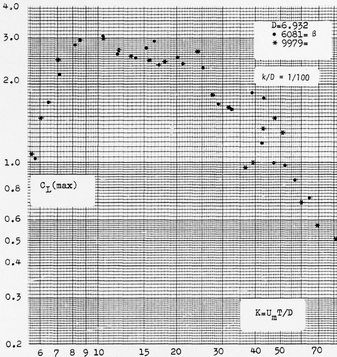
Figure 14. C_L(\max) versus K for k/D = 1/100 , 7 inch.
