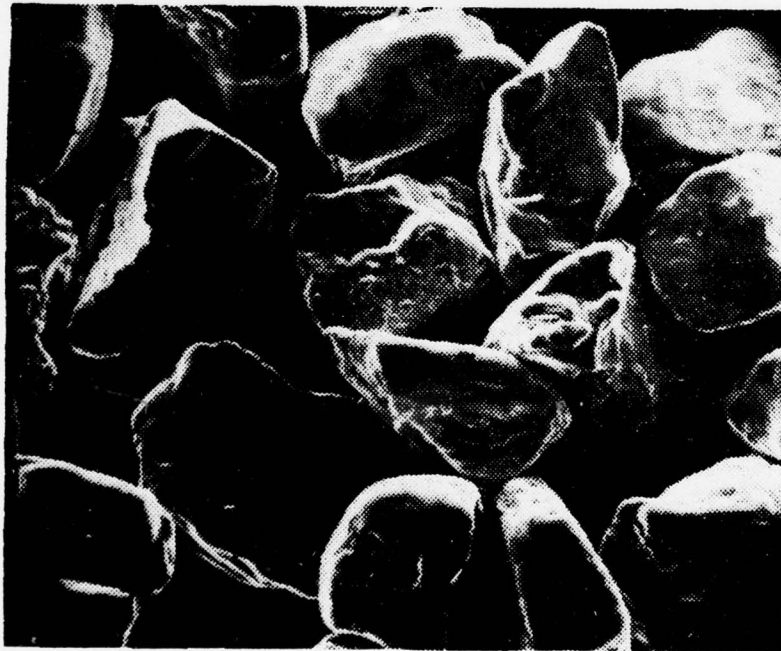
Figure 3. Scanning electron microscope photographs of sand-roughened surface.
