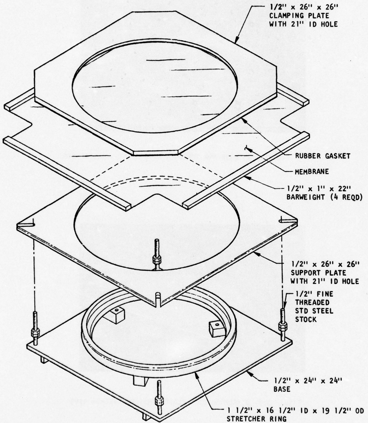
FIGURE 3-1. ATC MEMBRANE TENSION RIG
