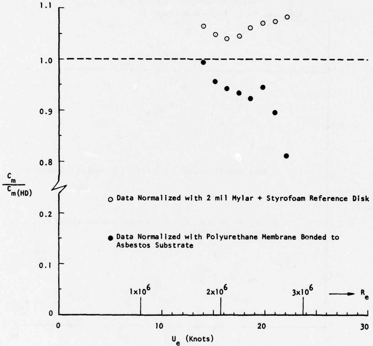
FIGURE 4-18. NORMALIZED MOMENT COEFFICIENT DATA
