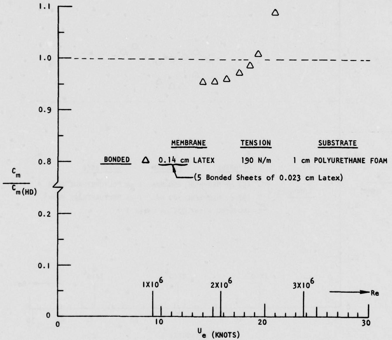
FIGURE 4-14. NORMALIZED MOMENT COEFFICIENT DATA
