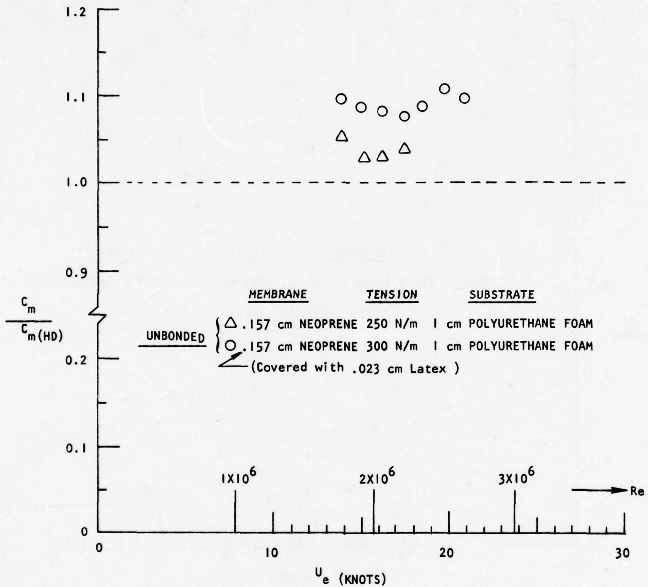
FIGURE 4-15. NORMALIZED MOMENT COEFFICIENT DATA
