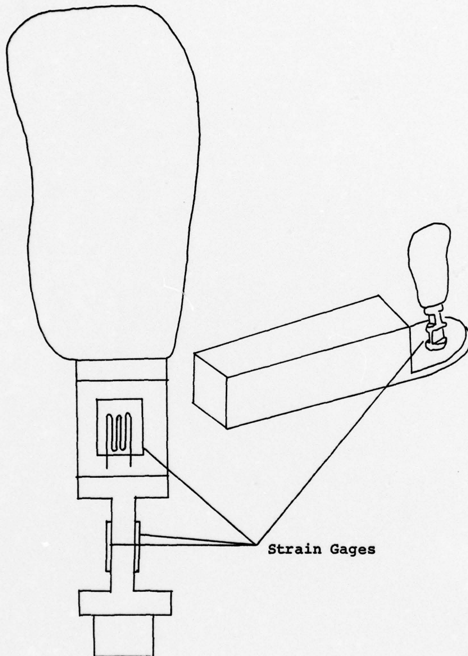
Figure 9. Side-Arm Force Stick Strain Gages.
