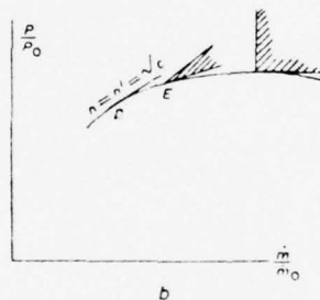
STABLE WHEN n' LIES IN THE SHADED AREA
