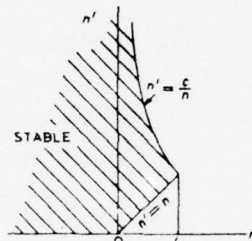
n SLOPE OF COMPRESSOR CHARACTERISTIC
