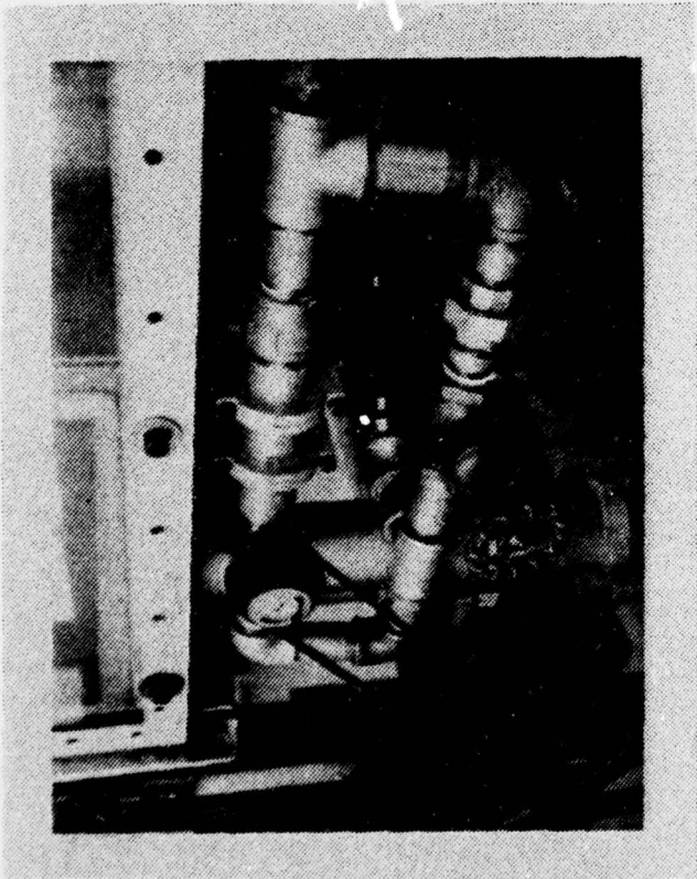
Figure 2a. Air enters through the rubber hose section at the rear. The rotating control valve is in the upper left corner and the bypass globe valve is in the lower center. Air exits at the right and is then ducted to the airfoil.
