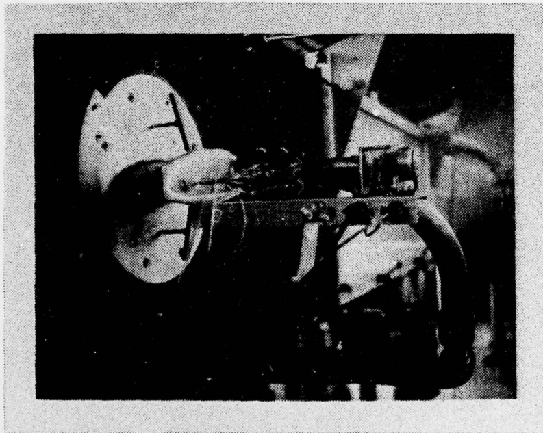
Figure 4 Scanivalve Mount
