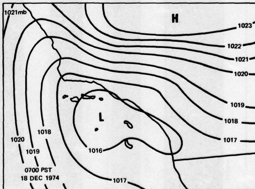
Figure 25. Mesoscale analysis of the sea-level pressure at 0700 PST on 18 December 1974.
