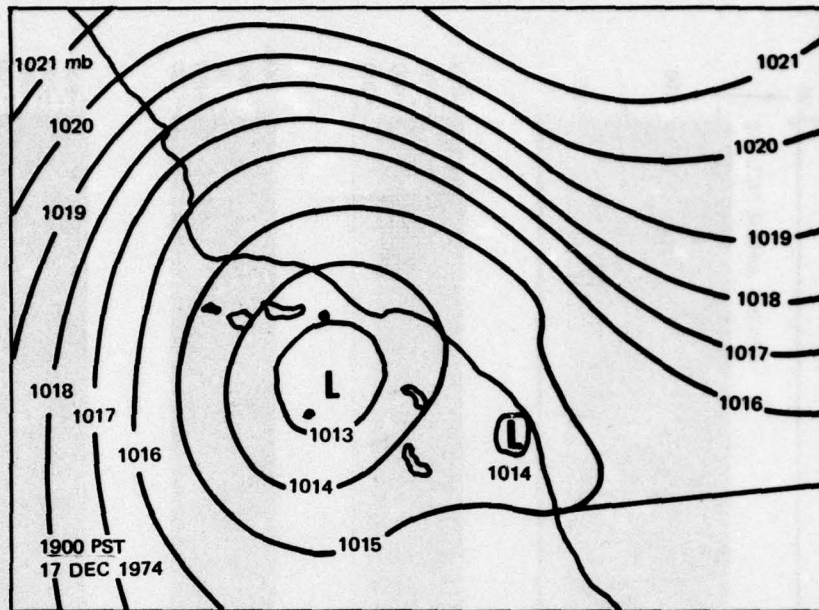
Figure 24. Mesoscale analysis of the sea-level pressure at 1900 PST on 17 December 1974.
