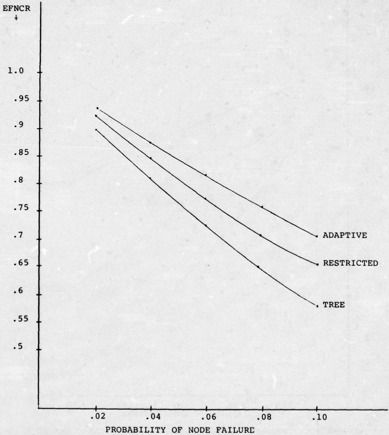
FIGURE 4.5: EXPECTED FRACTION OF NODE PAIRS THAT CAN COMMUNICATE THROUGH THE ROOT AS A FUNCTION OF NODE FAILURE, FOR DIFFERENT ROUTING ALGORITHMS AND FOR A NETWORK WITH A ROOT NODE IN CORNER
