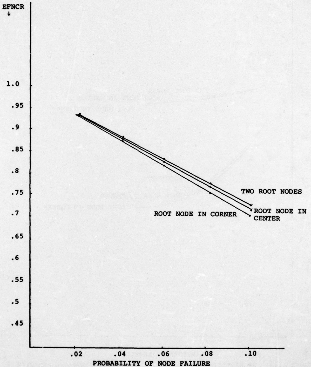
FIGURE 4.16: EXPECTED FRACTION OF NODE PAIRS THAT CAN COMMUNICATE THROUGH THE ROOT FOR ADAPTIVE ROUTING AS A FUNCTION OF NODE FAILURE FOR DIFFERENT NETWORK TOPOLOGIES
