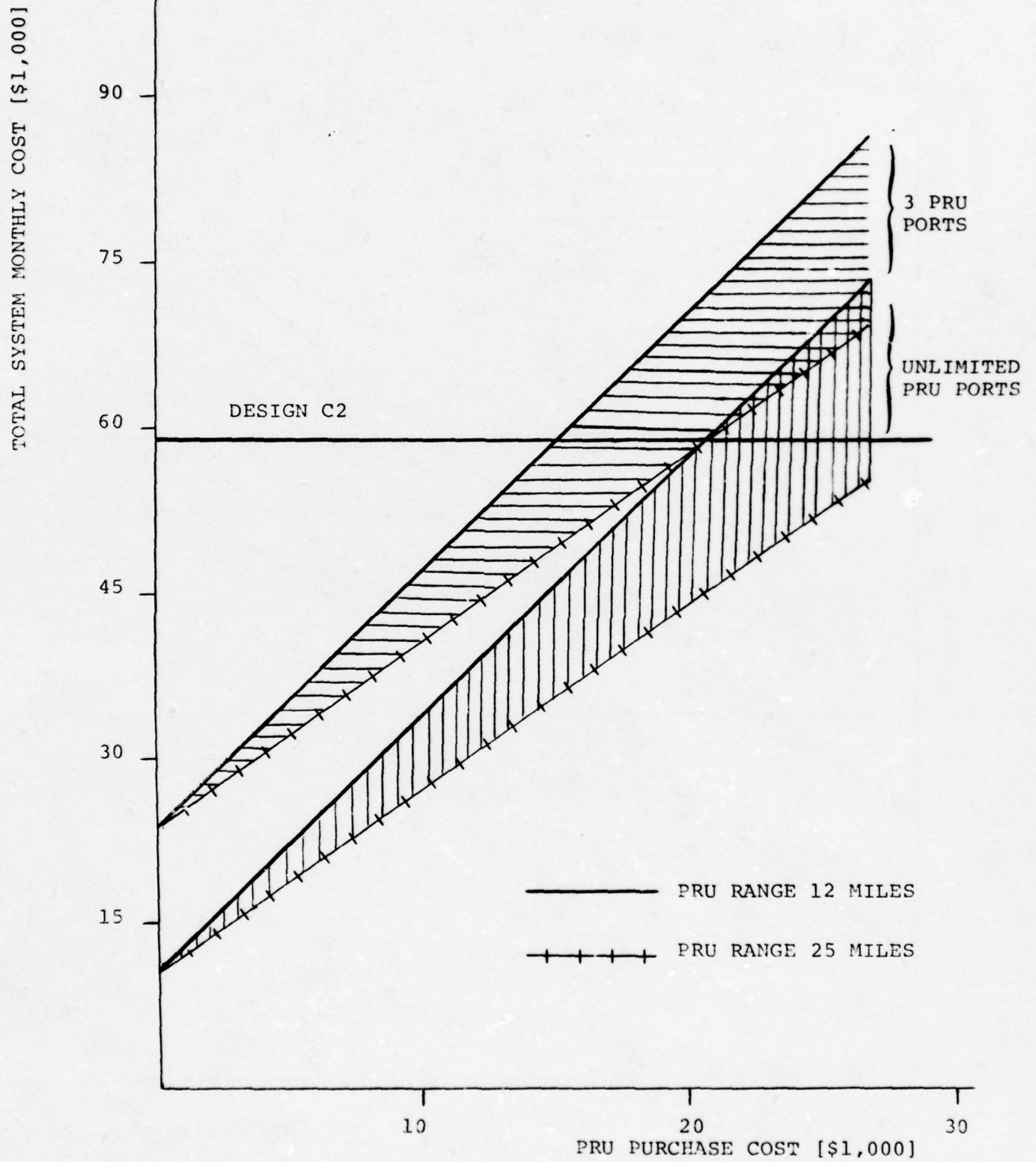
FIGURE 2.6: MONTHLY SYSTEM COST FOR ALTERNATIVE DESIGNS WITH DUAL HOMING RELIABILITY
