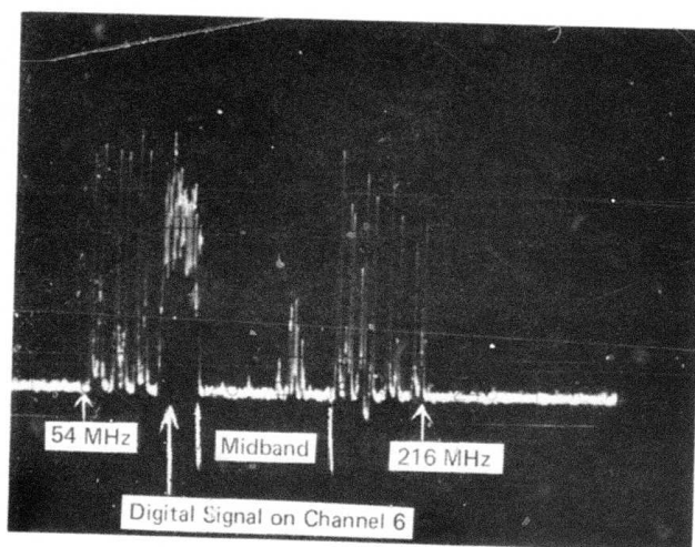
FIGURE 4.5a: FULL VIDEO SPECTRUM AND DIGITAL SIGNAL
