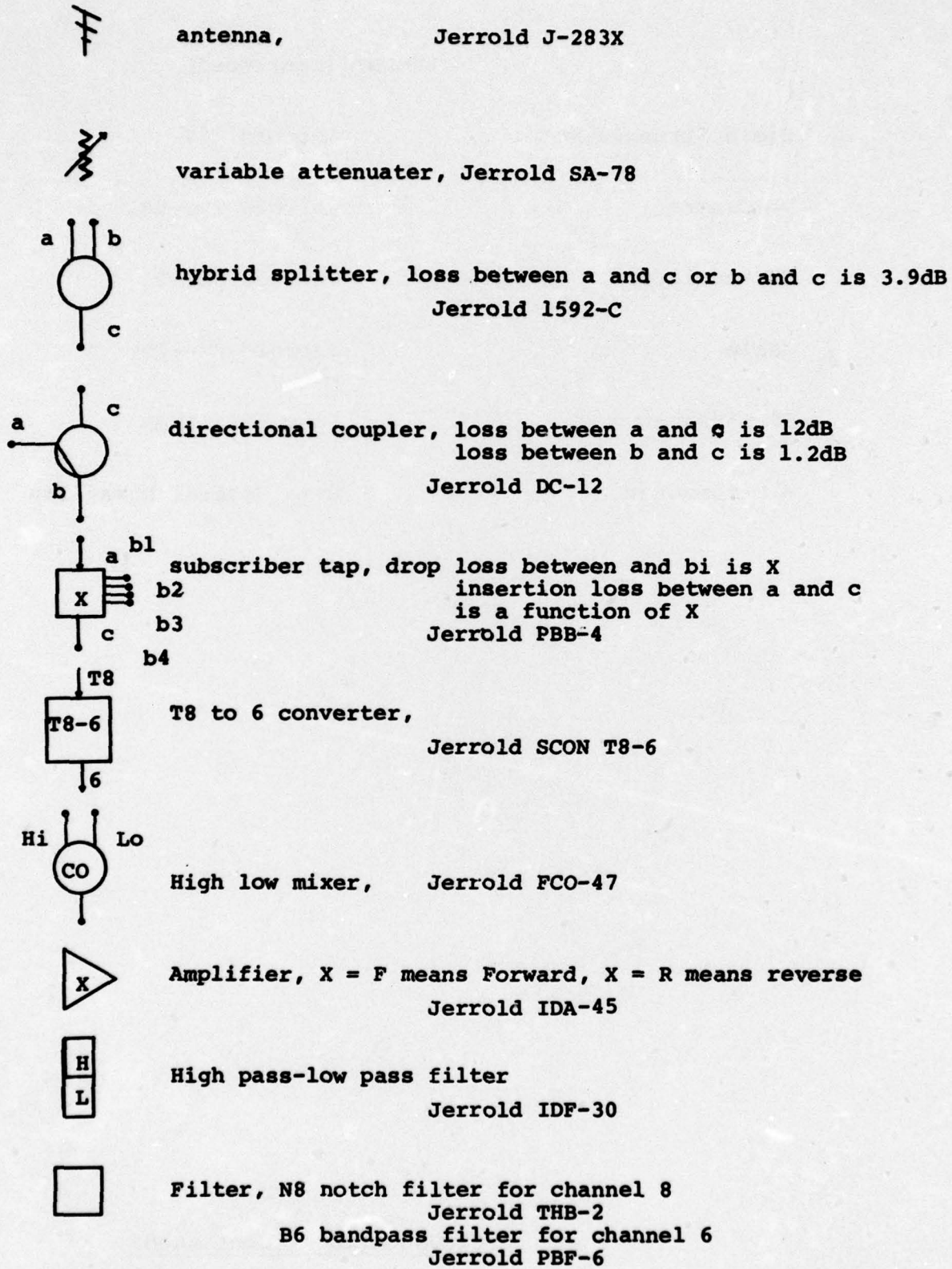
FIGURE 4.1c: LEGEND FOR SYSTEM CONFIGURATION
