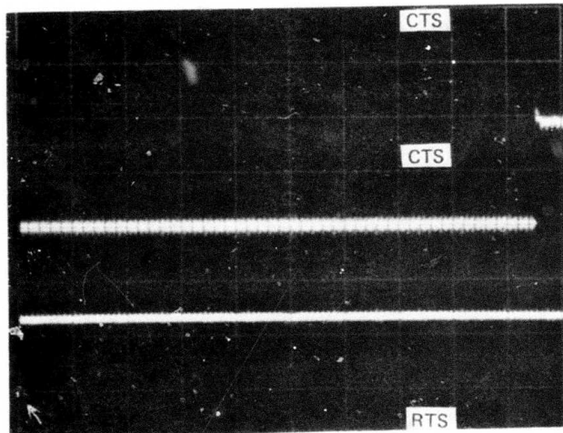
FIGURE 4.7b: CLEAR-TO-SEND (UPPER SIGNAL) 96 μSEC. AFTER REQUEST-TO-SEND (LOWER SIGNAL) 10 μSEC/CM.
