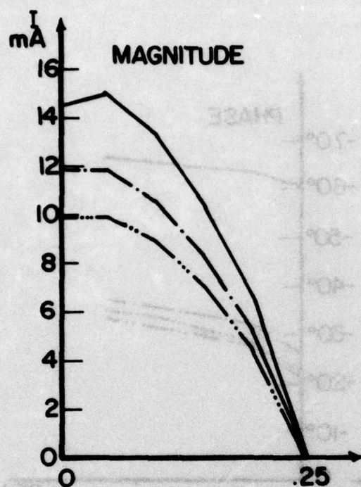
(a) .25\lambda DRIVEN WIRE
