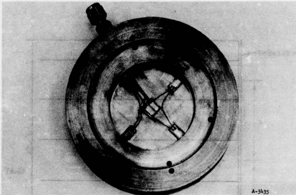
Figure 22. WES earth pressure cell with cover plate removed
