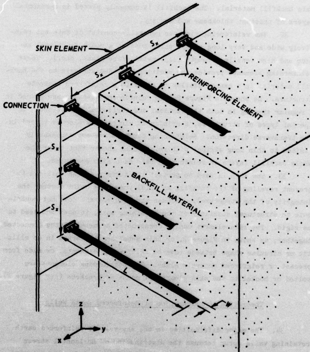
Figure 2. Schematic of major elements of reinforced earth wall
