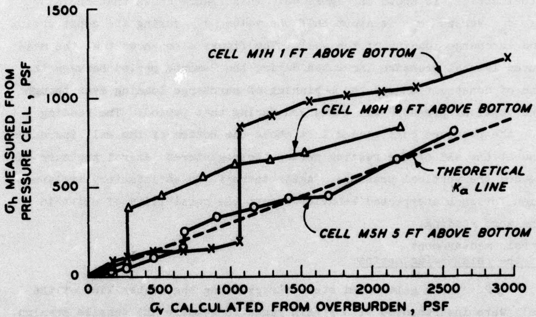
Figure 42. Comparison between the measured horizontal stress and the calculated vertical stress for wall reinforced with galvanized steel strips
