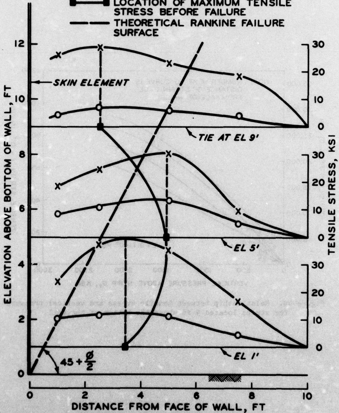
Figure 50. Tensile stress distribution along the instrumented reinforcing ties at the end of construction and before failure
