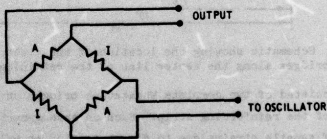
b. COMPLETE BRIDGE
