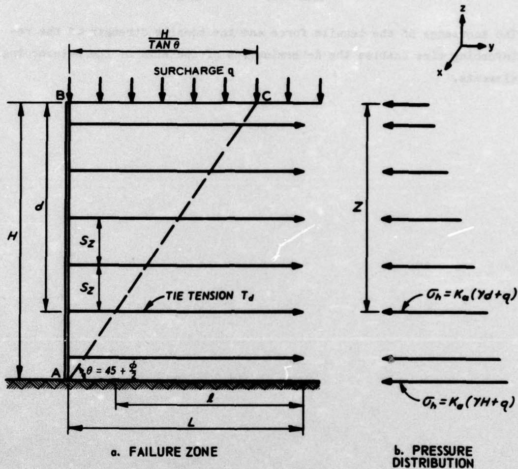
Figure 5. Pressure distribution according to Rankine theory
